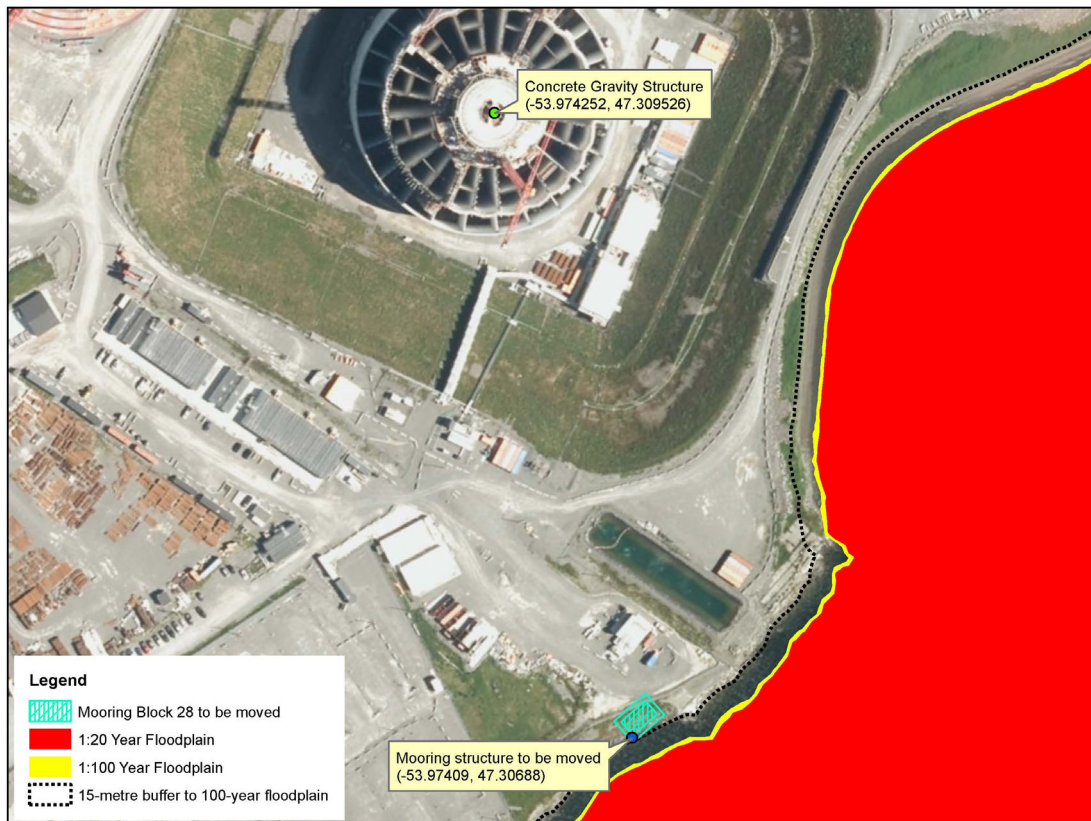
Relocation of a Mooring Block into 15 metres boundary of 1:100 year floodplain
