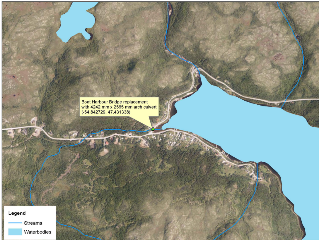
Boat Harbour Bridge replacement with Arch Culvert
