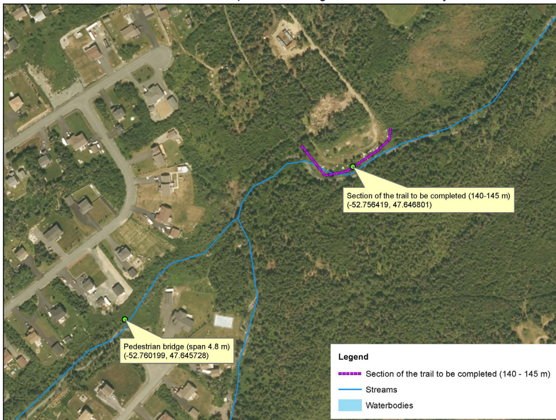
Trail construction and pedestrian bridge installation in Torbay
