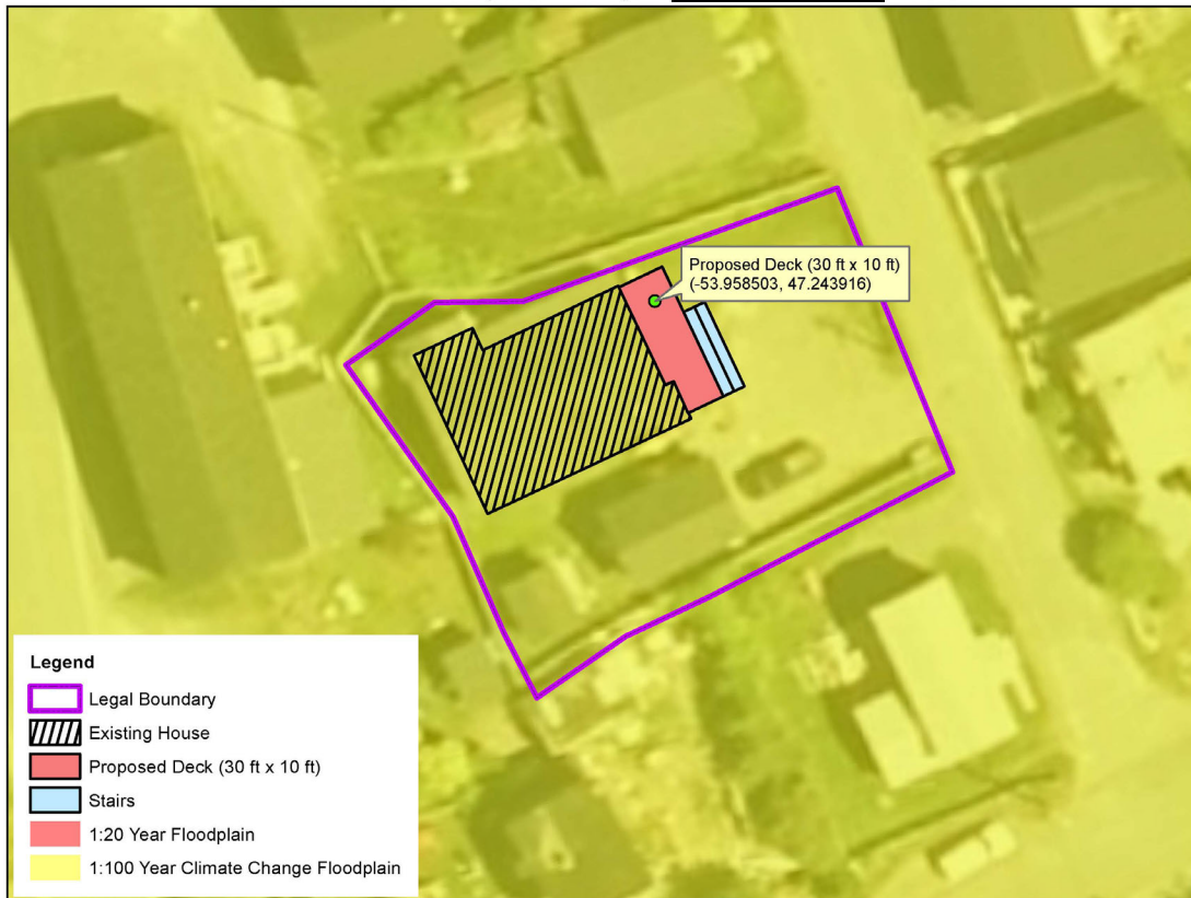
Construction of a Deck (30 ft x 10 ft) at [REDACTED] Placentia
