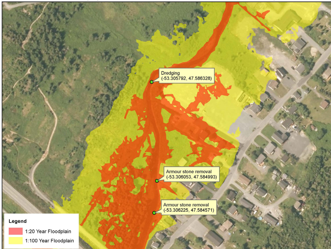
Location 1 - Dredging and Armour Stone removal in Shearstown Brook, Bay Roberts
