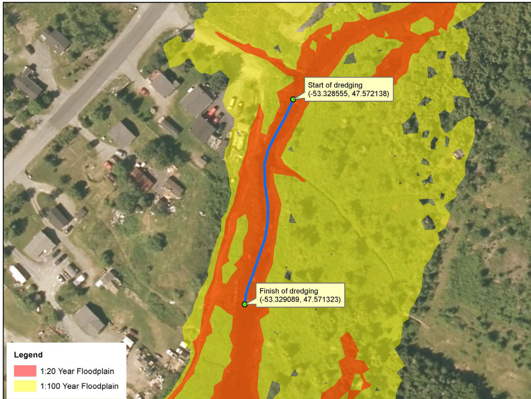
Location 2 - Dredging in Shearstown Brook, Bay Roberts
