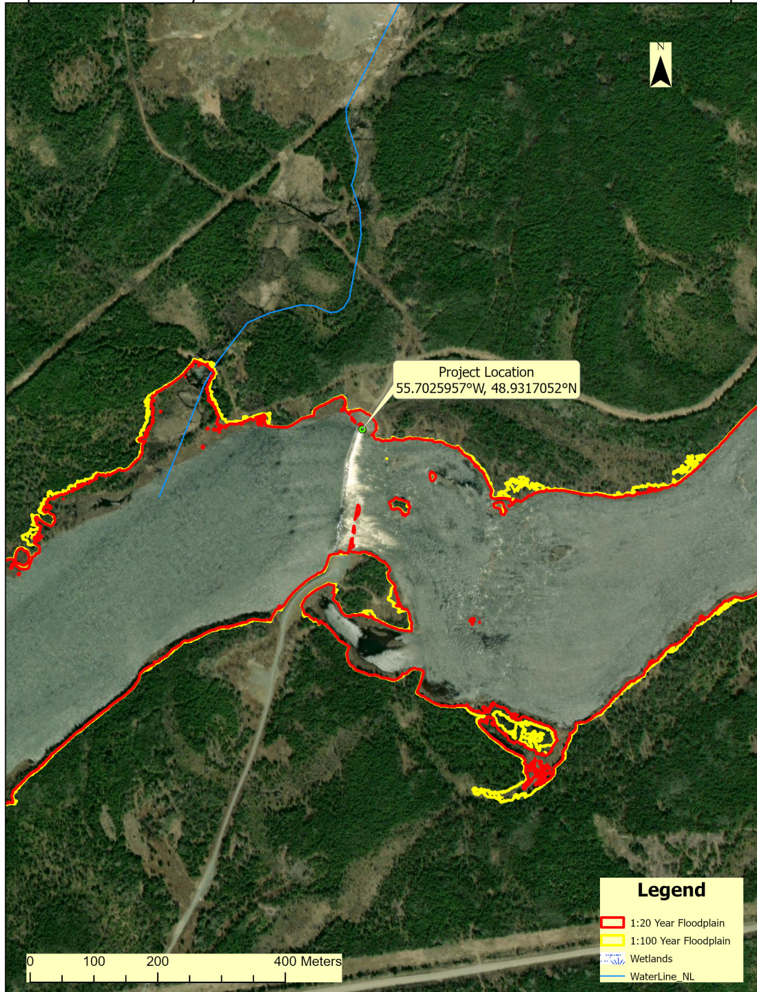
Exploits River - Goodyears Dam - Salmon Ladder Debris Removal and Concrete Repair
