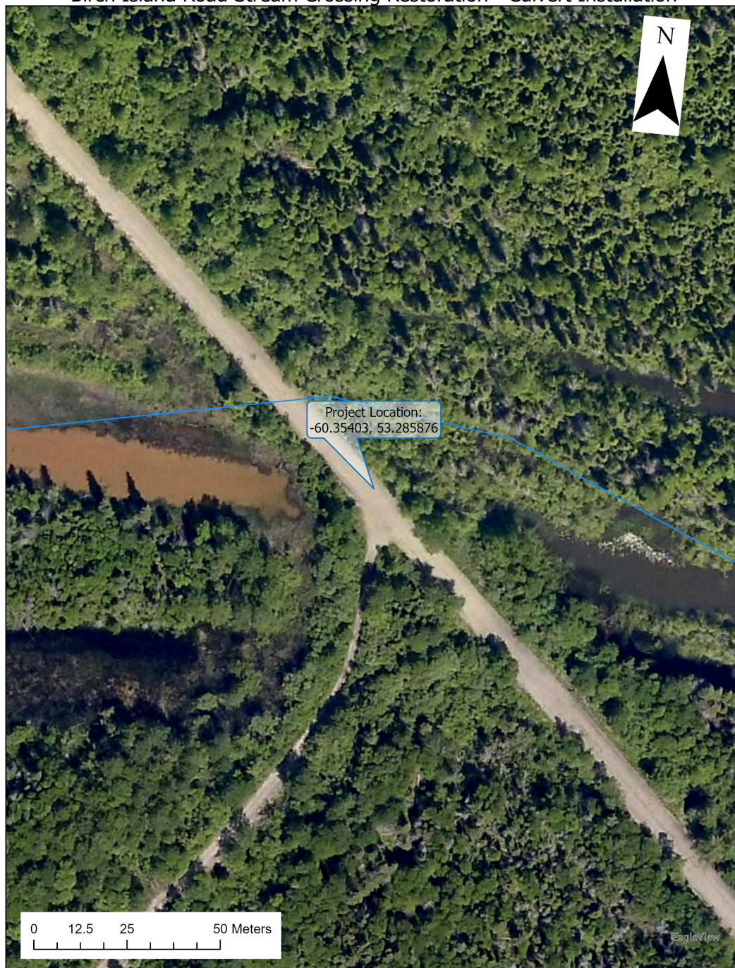
Birch Island Road Stream Crossing Restoration - Culvert Installation
