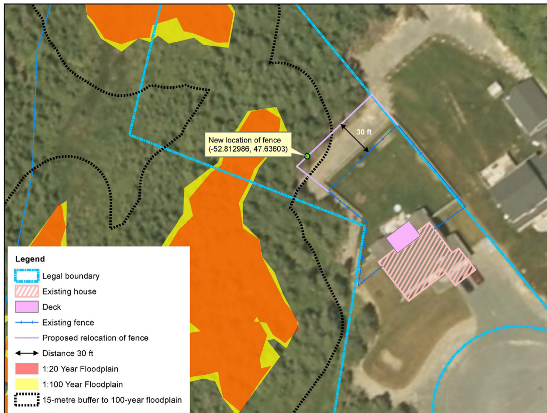
Fence relocation at 52 Jera Street, Portugal Cove-St. Philip's
