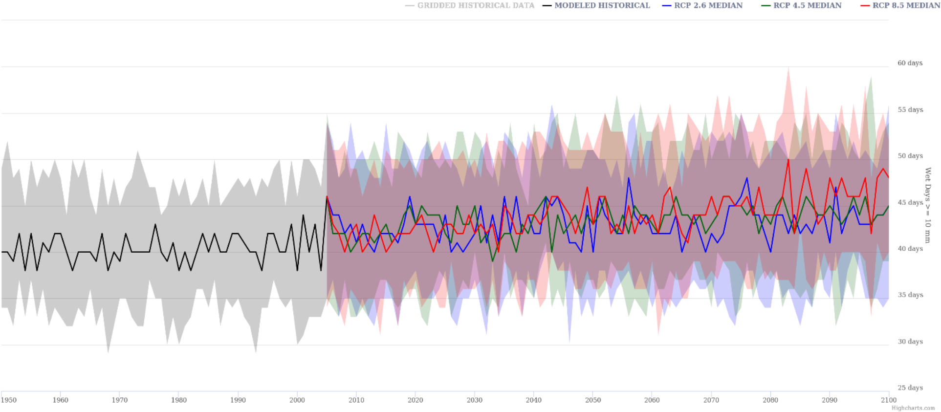
Figure 5 Wet Days ≥ 10 mm Climate Change Projection.
