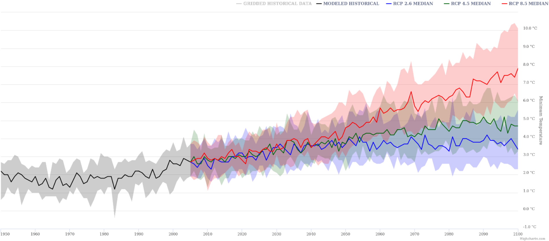
Figure 3 Minimum Temperature Climate Change Projection.
