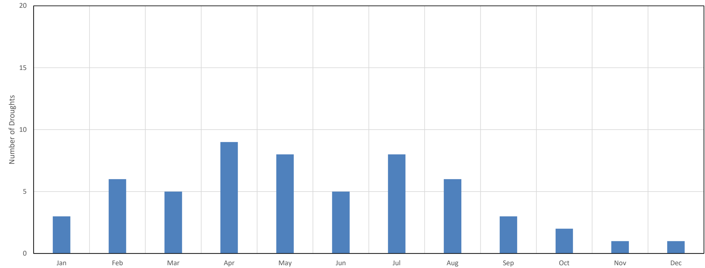
Annual Drought Distribution
