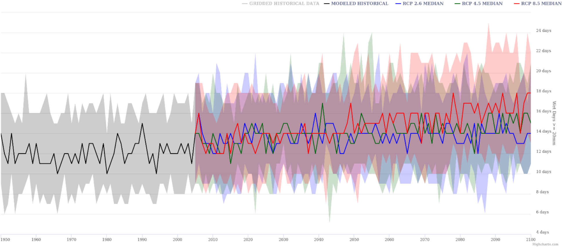
Figure 6 Wet Days ≥ 20 mm Climate Change Projection.
