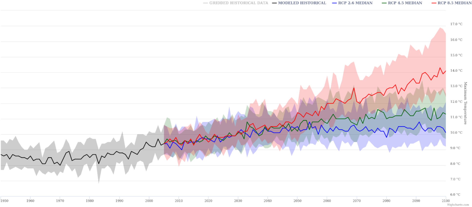
Figure 4 Maximum Temperature Climate Change Projection.
