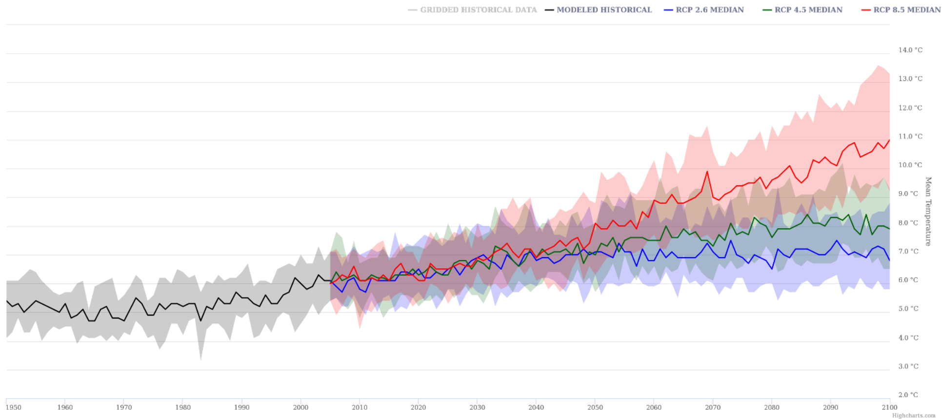
Figure 2 Mean Temperature Climate Change Projection.
