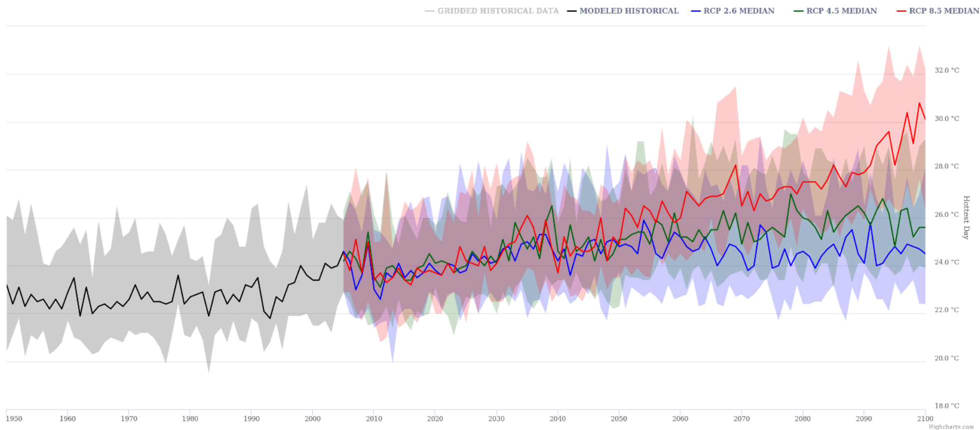
Figure 1 Hottest Day Climate Change Projection.
