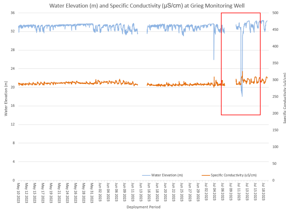
Figure 10: Water Elevation (m) and Specific Conductivity ( \mu\text{S}/\text{cm} ) at Grieg Monitoring Well. The red box indicates a sharp decrease in water elevation (likely due to pumping), followed by an increase in specific conductivity.
