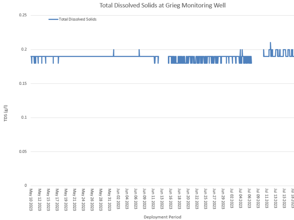
Figure 9: Total Dissolved Solids (TDS)
