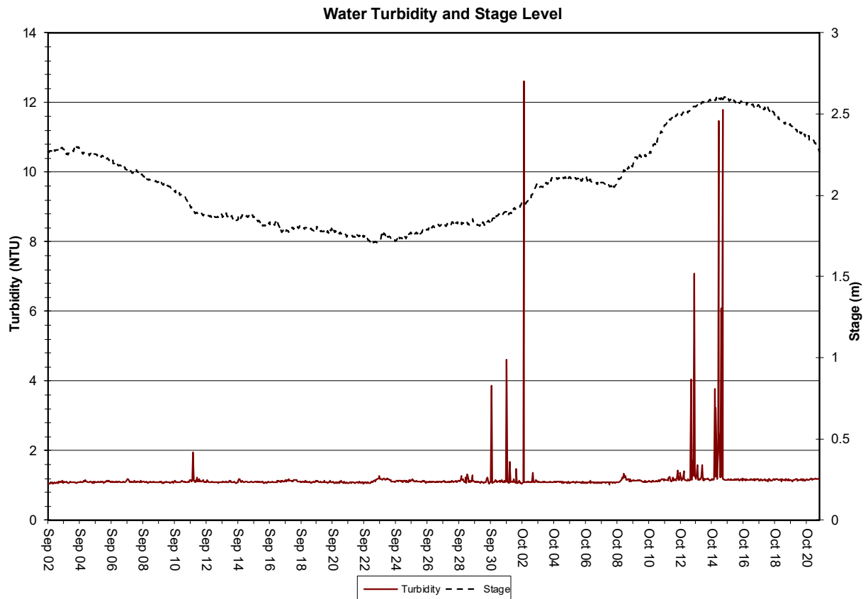
Figure 6: Turbidity (NTU) at Humber River from September 2 to October 21, 2020
