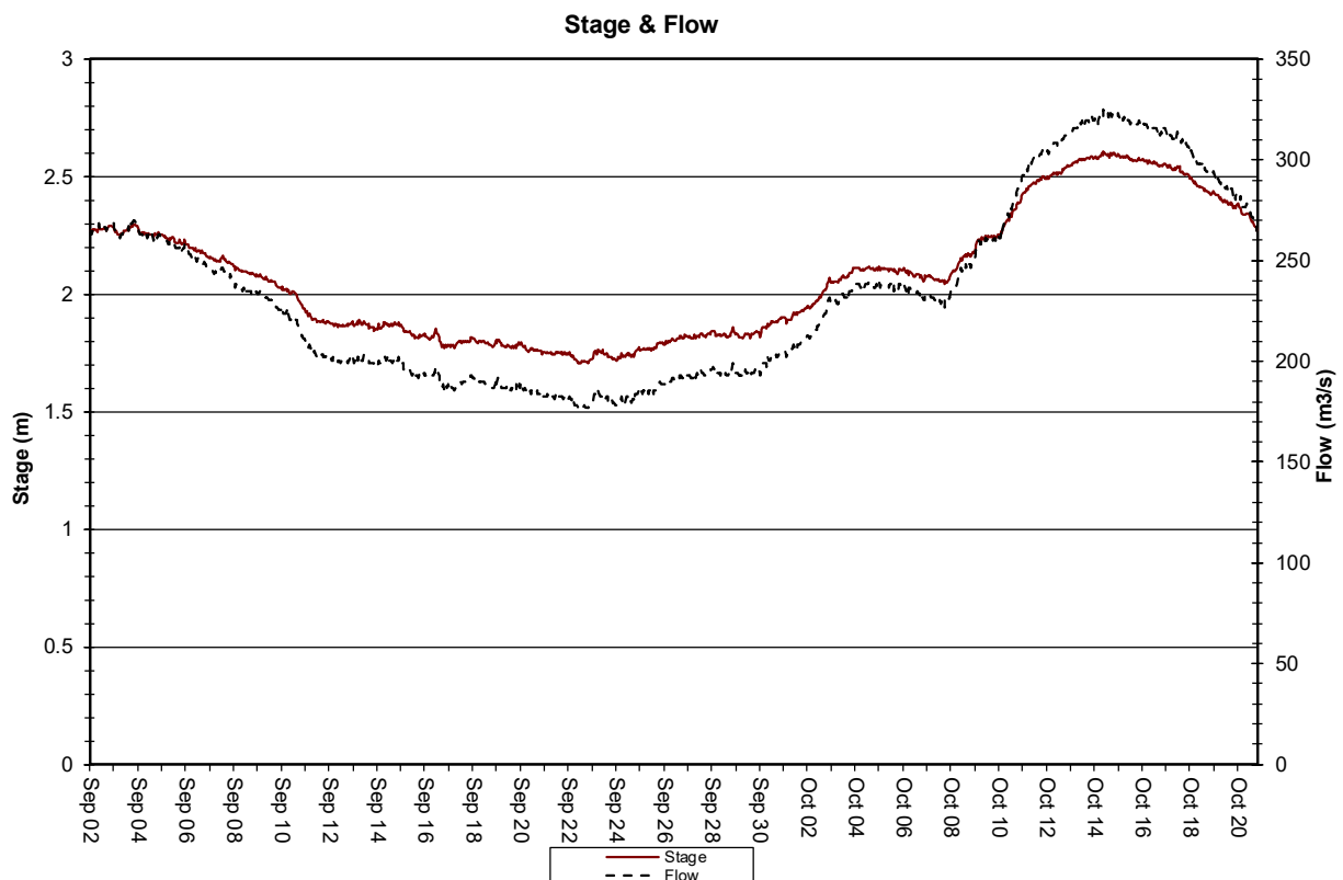
Figure 1: Stage & Flow at Humber River from September 2 to October 21, 2020
