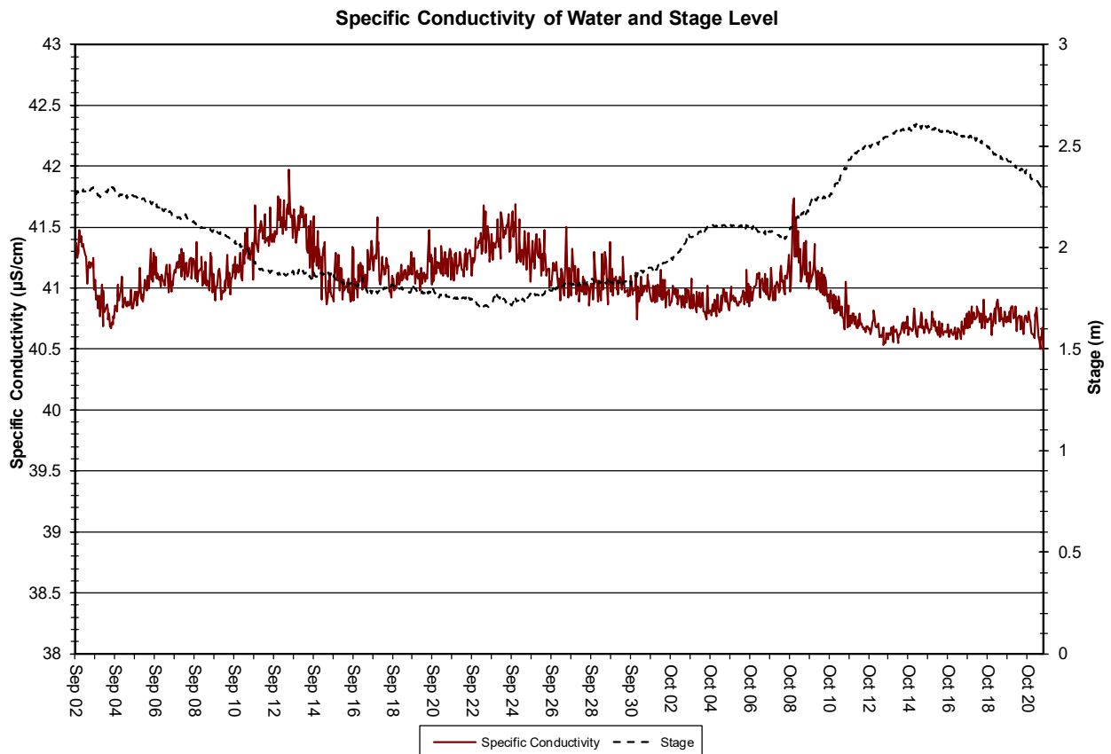
Figure 4: Specific conductivity ( \mu\text{S}/\text{cm} ) at Humber River from September 2 to October 21, 2020
