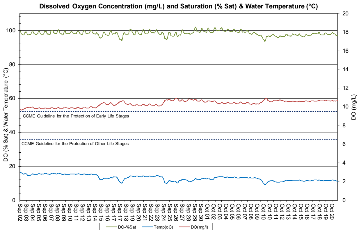
Figure 5: DO (mg/l & % saturation) at Humber River from September 2 to October 21, 2020
