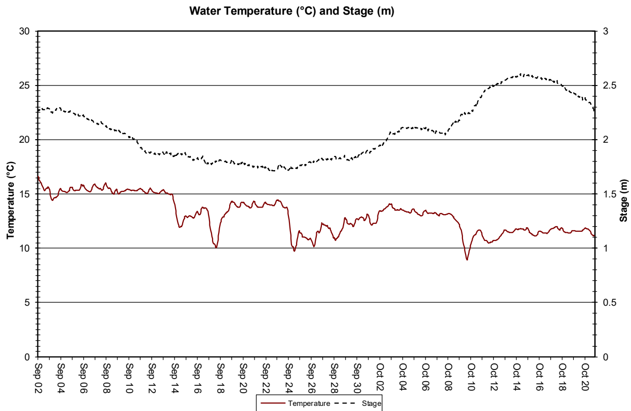
Figure 2: Temperature (°C) at Humber River from September 2 to October 21, 2020
