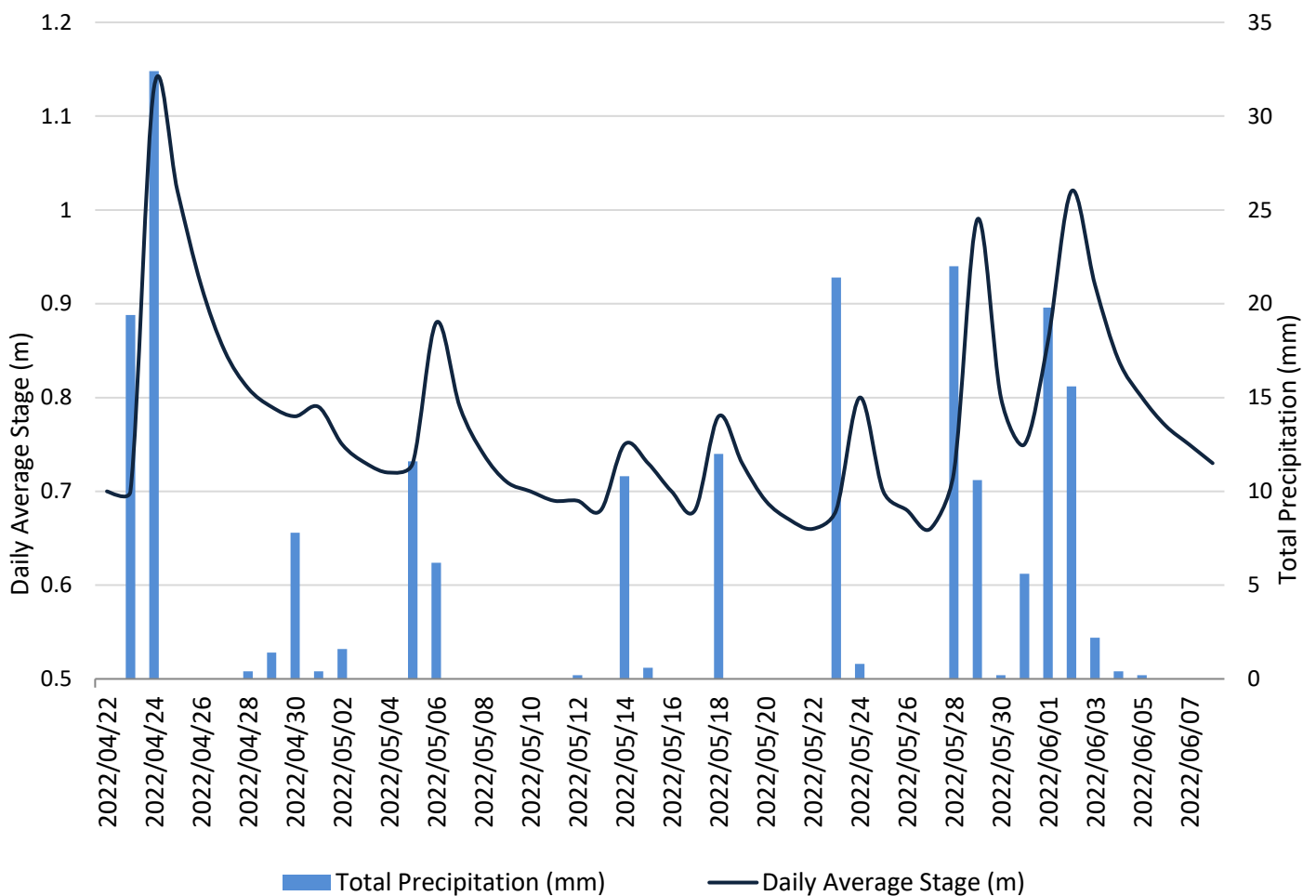
Figure 8 Daily average stage values (m) from Leary's Brook and daily total precipitation values (mm) from St. John's International Airport.
