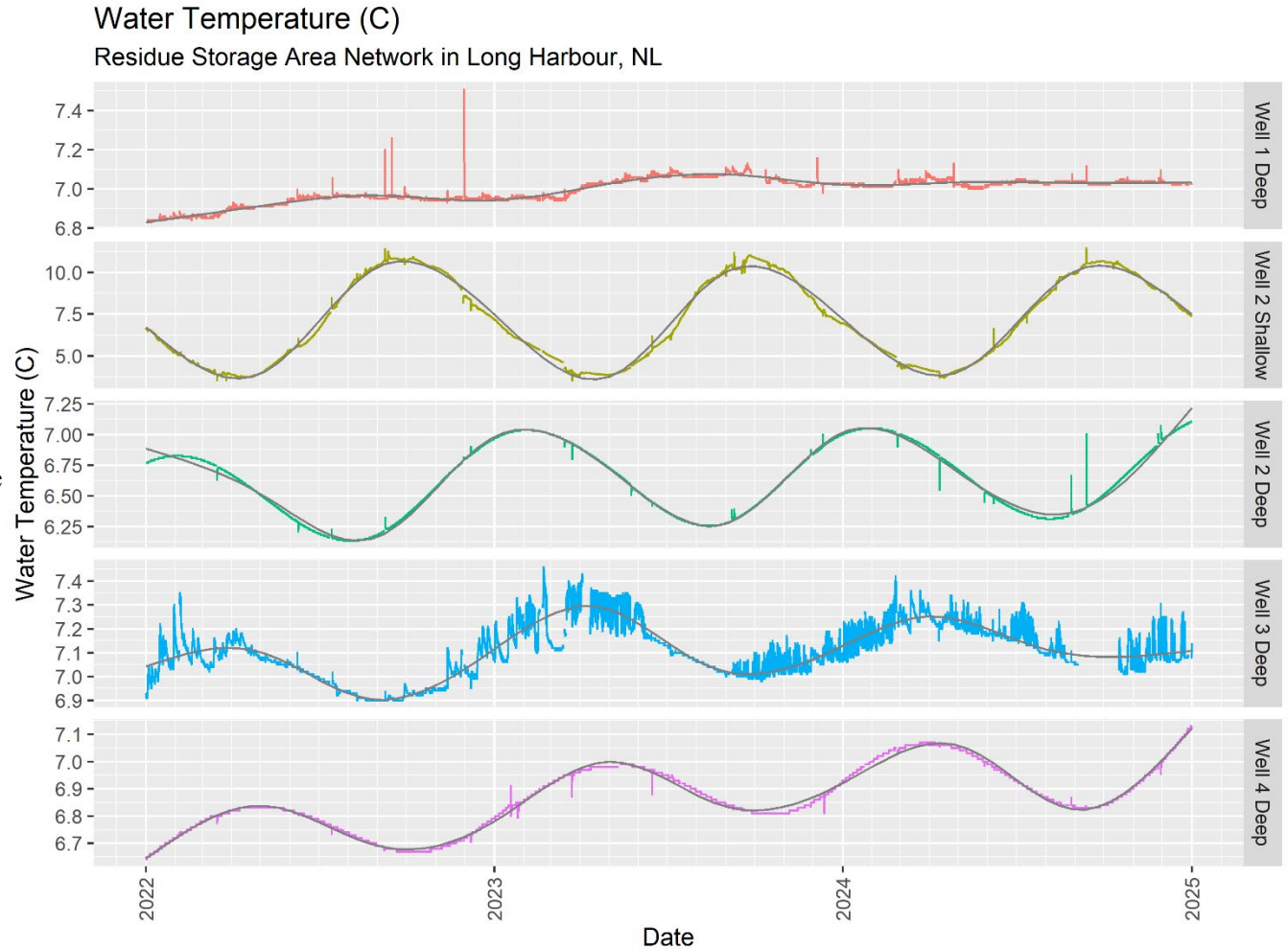
Figure 9: Water temperature at the Residue Storage Area from 2022 to 2024
