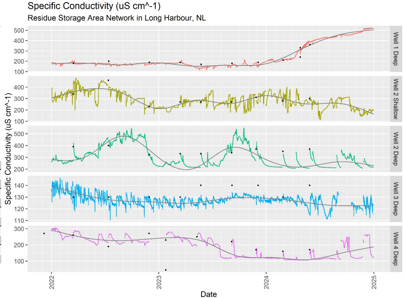
Figure 13: Specific conductivity at the Residue Storage Area from 2022 to 2024
