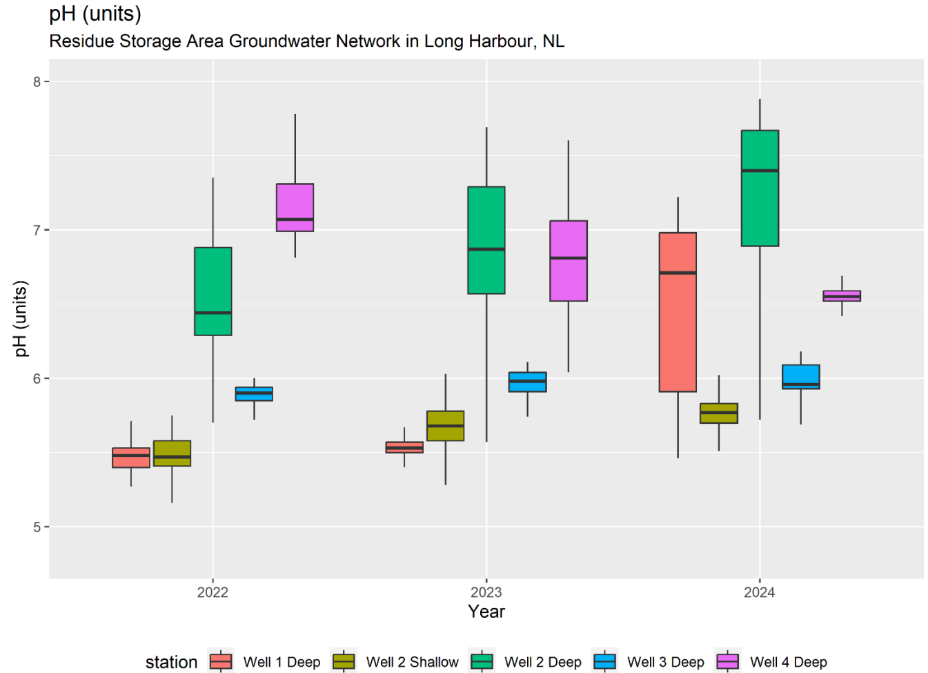
Figure 12: Boxplots of pH at the Residue Storage Area from 2022 to 2024
