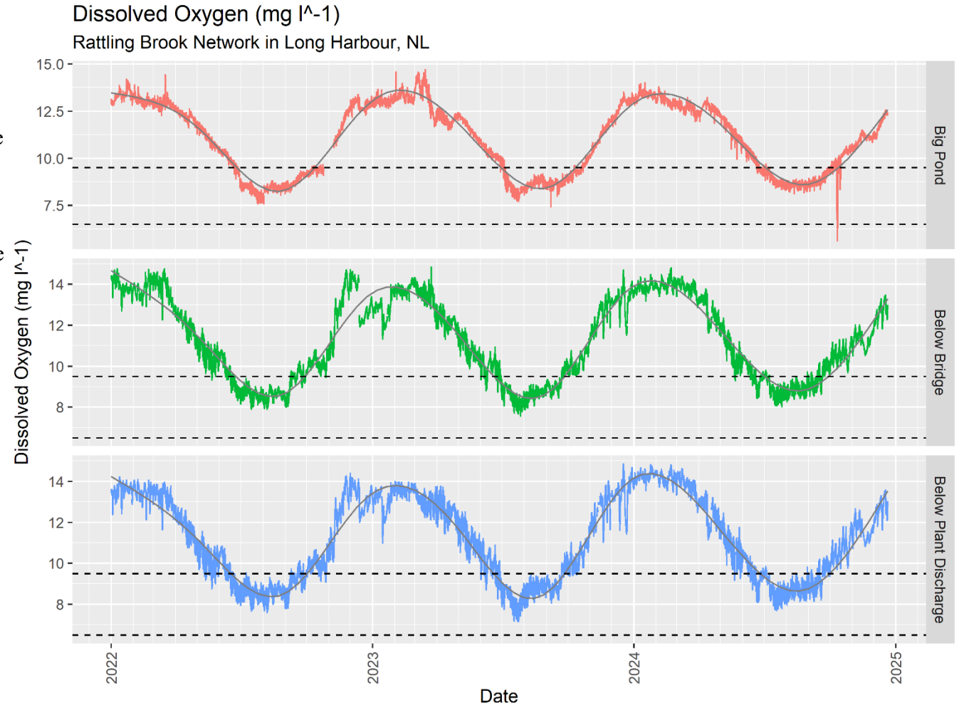
Figure 6: Dissolved oxygen at Rattling Brook from 2022 to 2024
