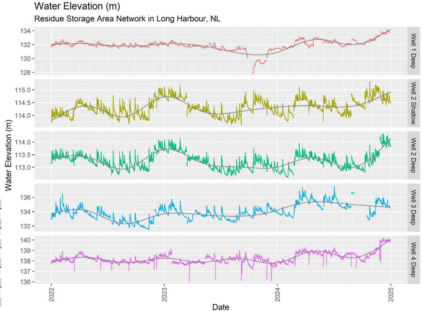
Figure 17: Water elevation at the Residue Storage Area from 2022 to 2024
