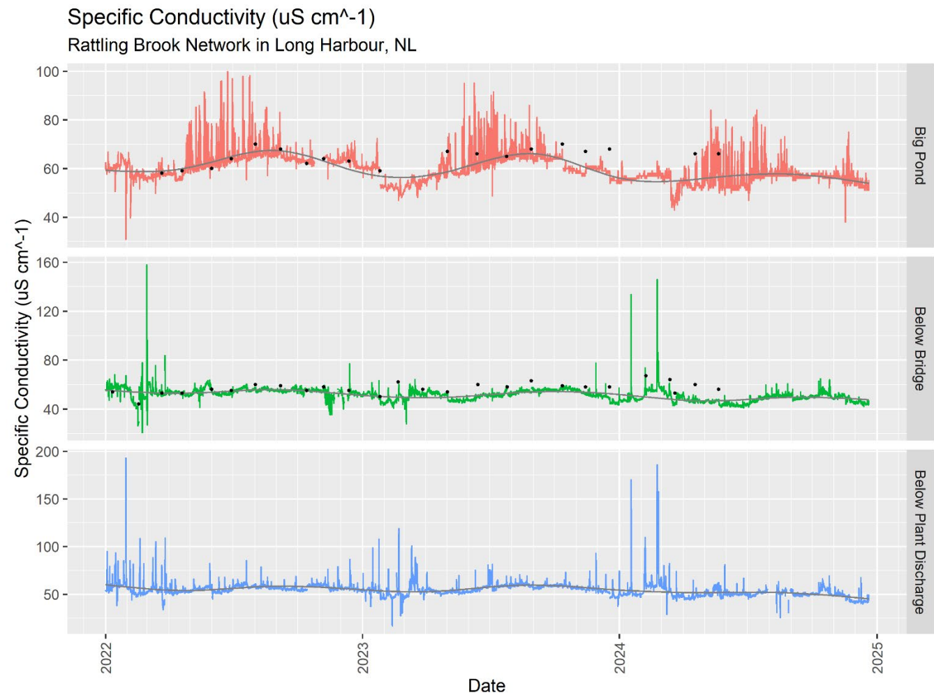
Figure 5: Specific Conductivity at Rattling Brook from 2022 to 2024
