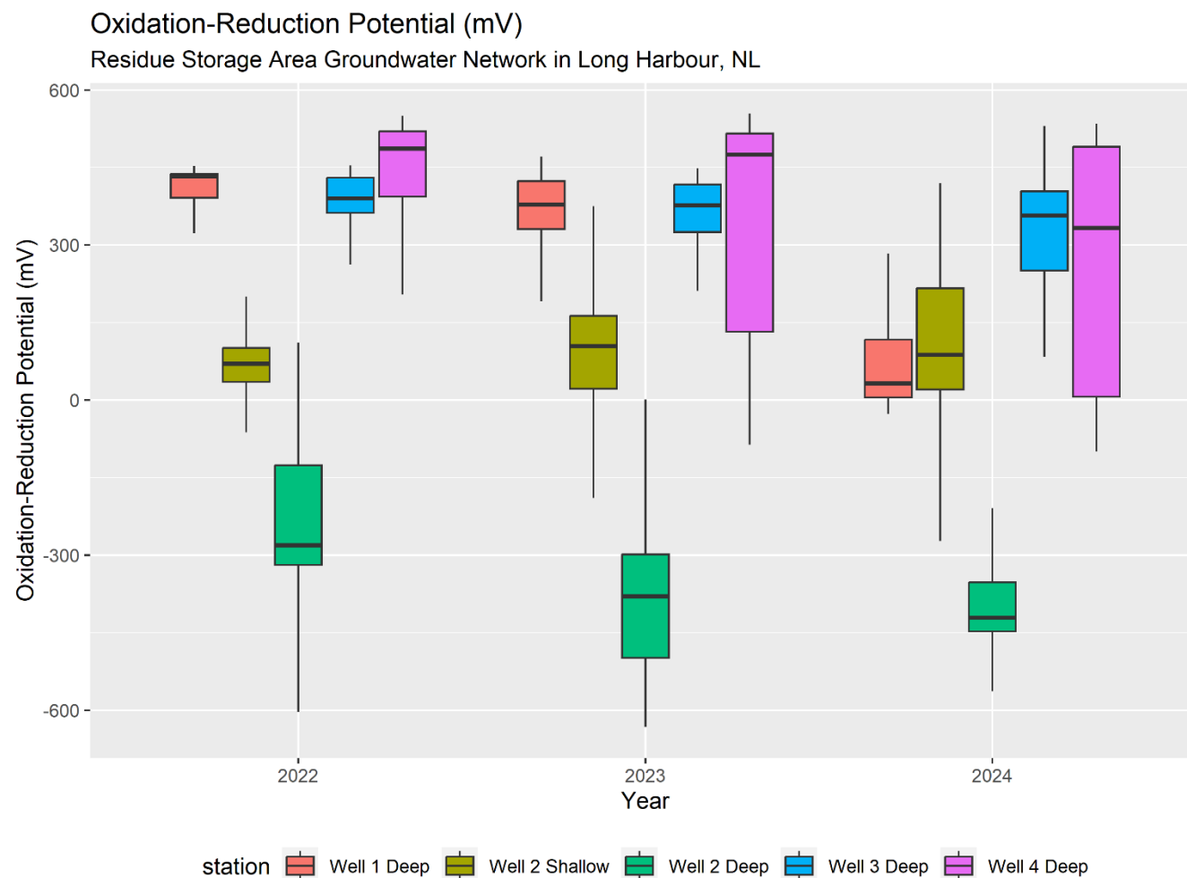
Figure 16: Boxplots of Oxidation-Reduction Potential at the Residue Storage Area from 2022 to 2024
