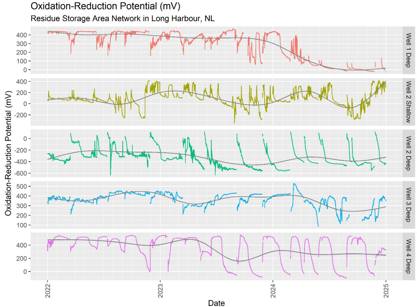
Figure 15: Oxidation-Reduction Potential at the Residue Storage Area from 2022 to 2024
