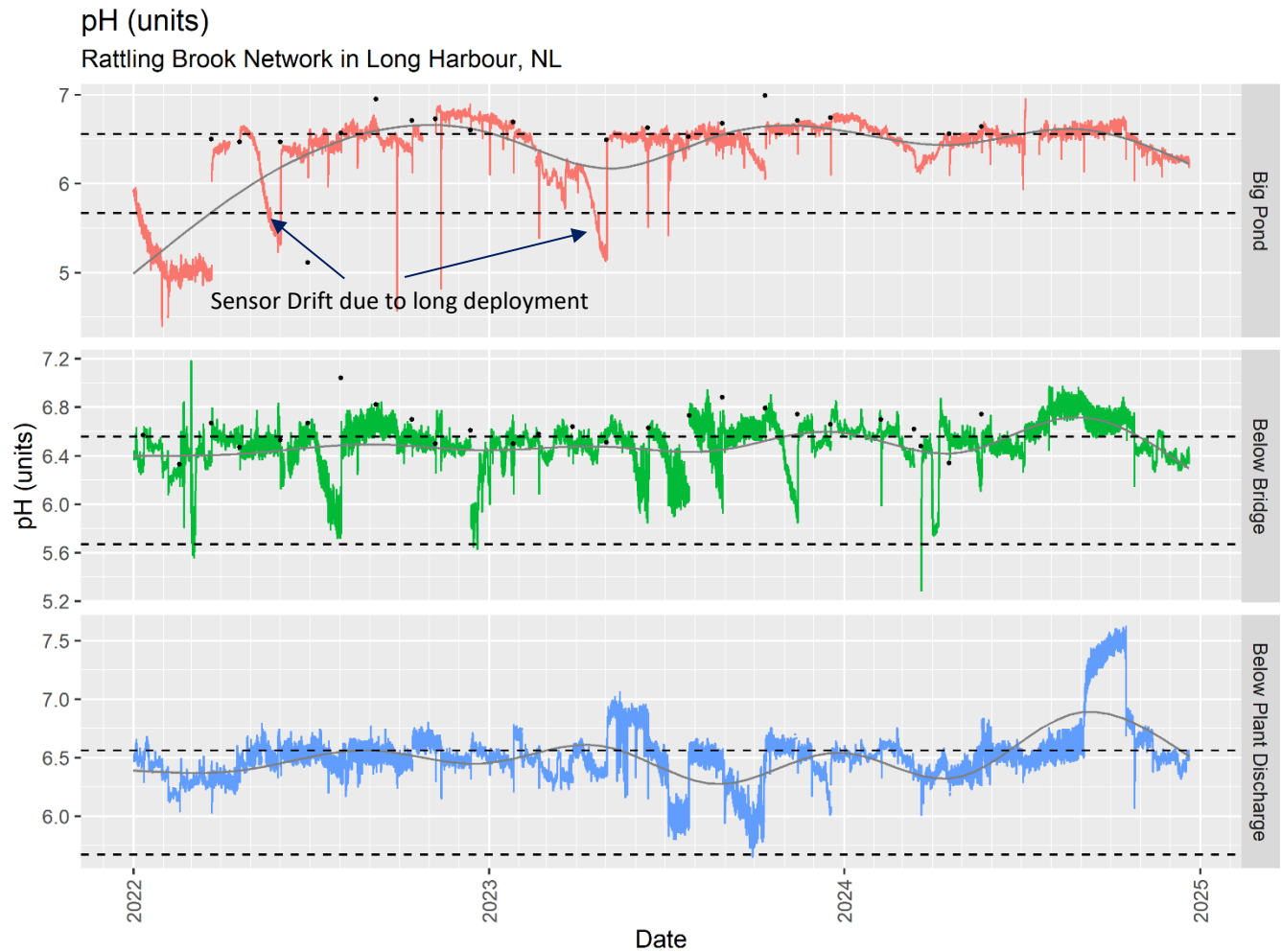
Figure 4: pH at Rattling Brook from 2022 to 2024
