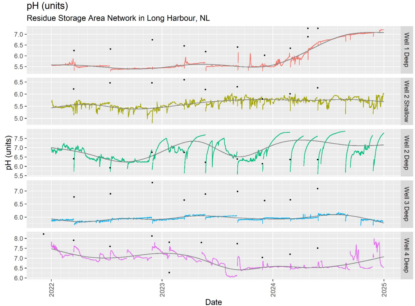
Figure 11: pH at the Residue Storage Area from 2022 to 2024
