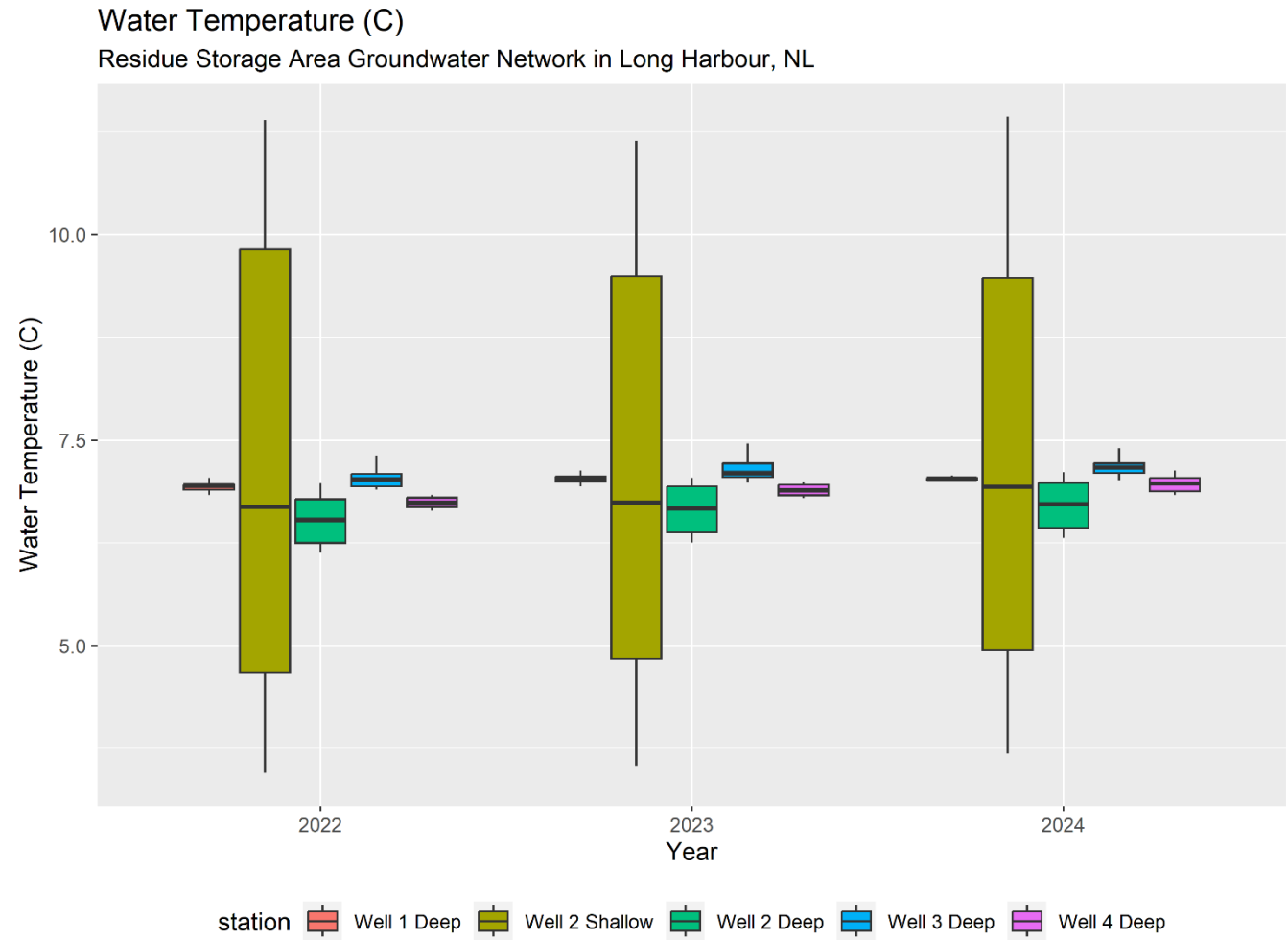
Figure 10: Boxplots of water temperature at the Residue Storage Area from 2022 to 2024
