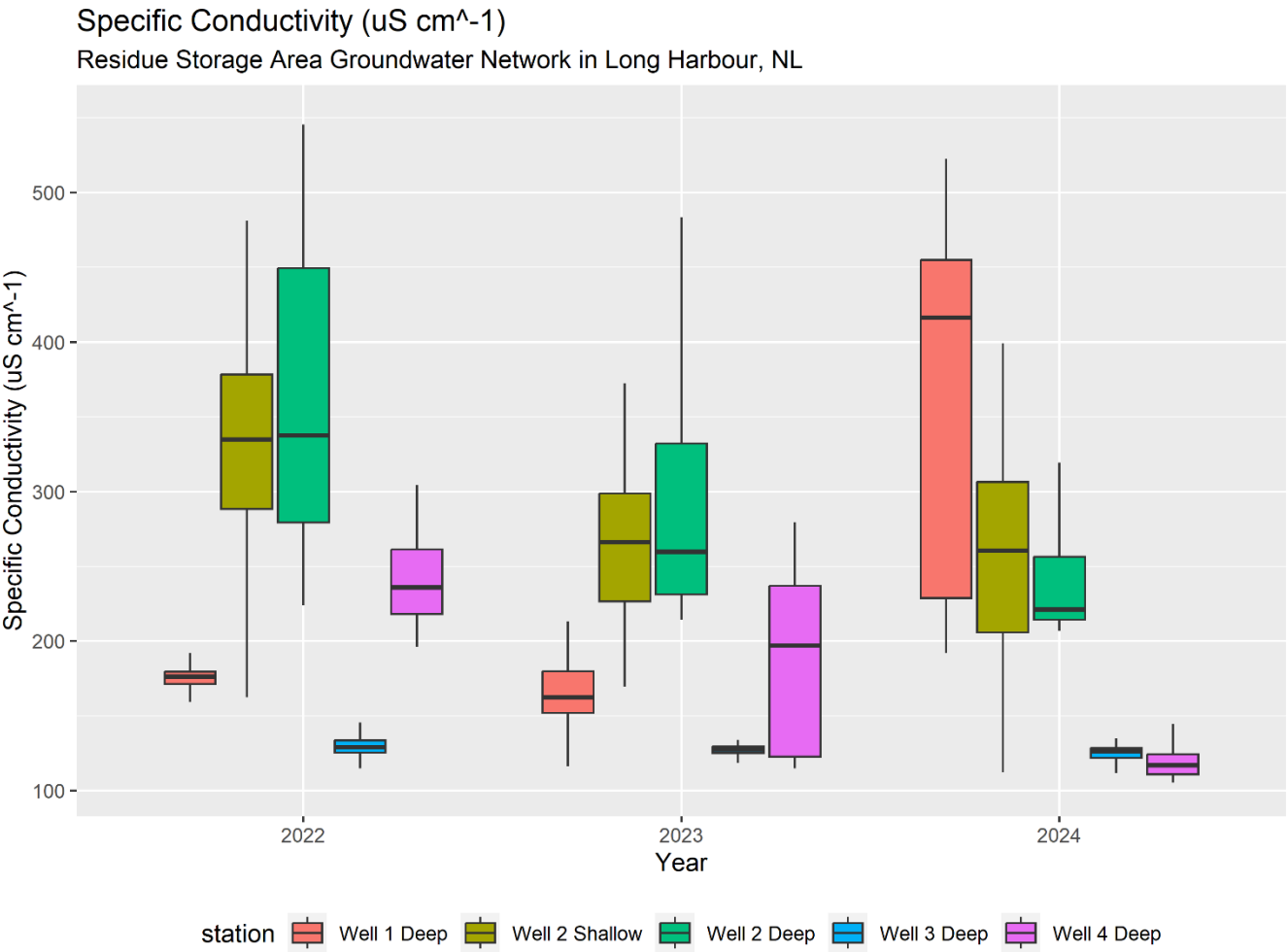
Figure 14: Boxplots of specific conductivity at the Residue Storage Area from 2022 to 2024
