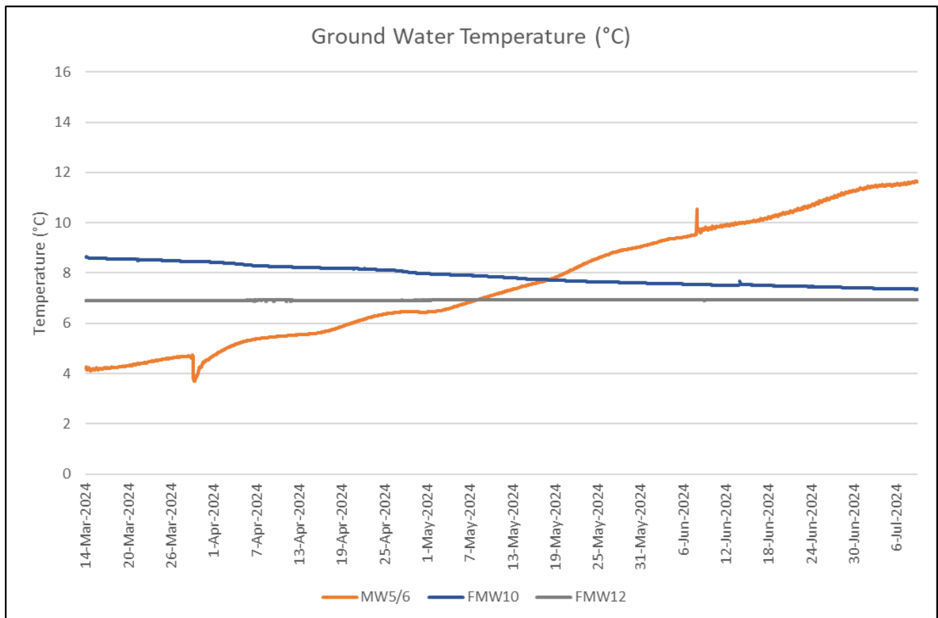
Figure 3: Ground Water Temperature (°C) – Northern Harvest Smolt Ltd. Network
