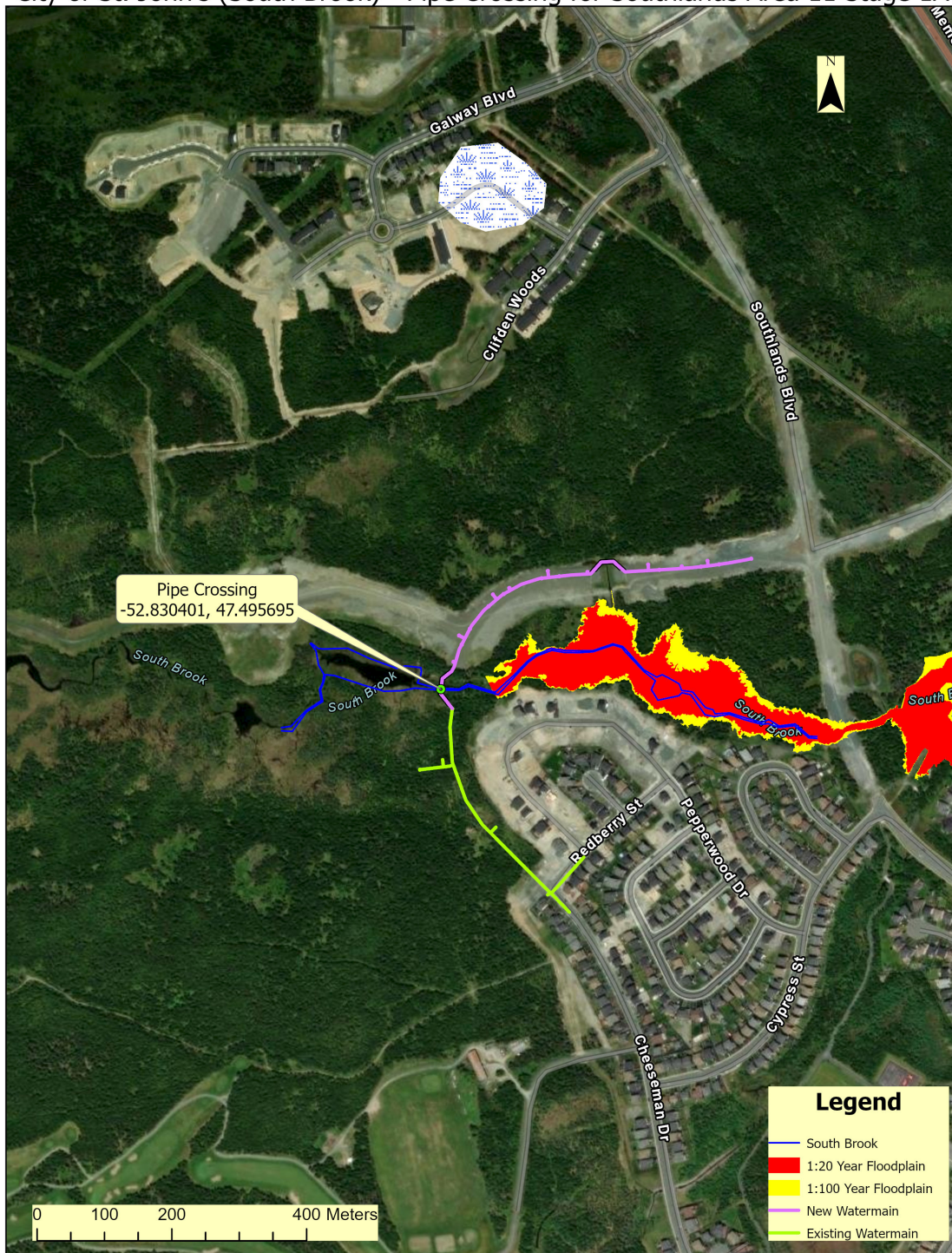
City of St. John's (South Brook) - Pipe Crossing for Southlands Area 11 Stage 1A
