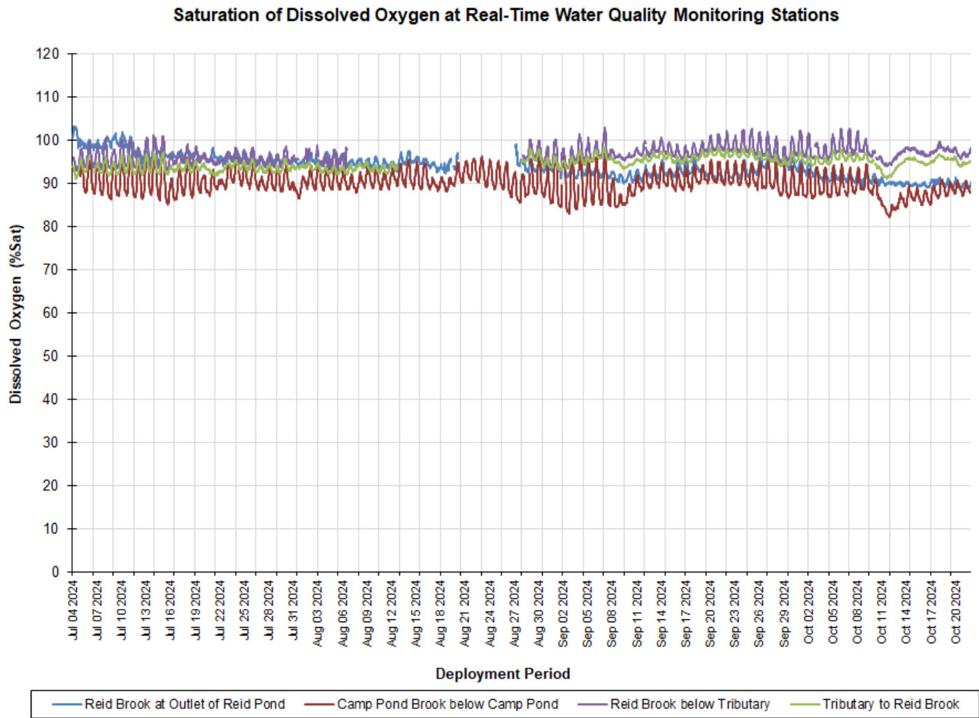
Figure 28b: Saturation of Dissolved Oxygen at all RTWQ Stations
