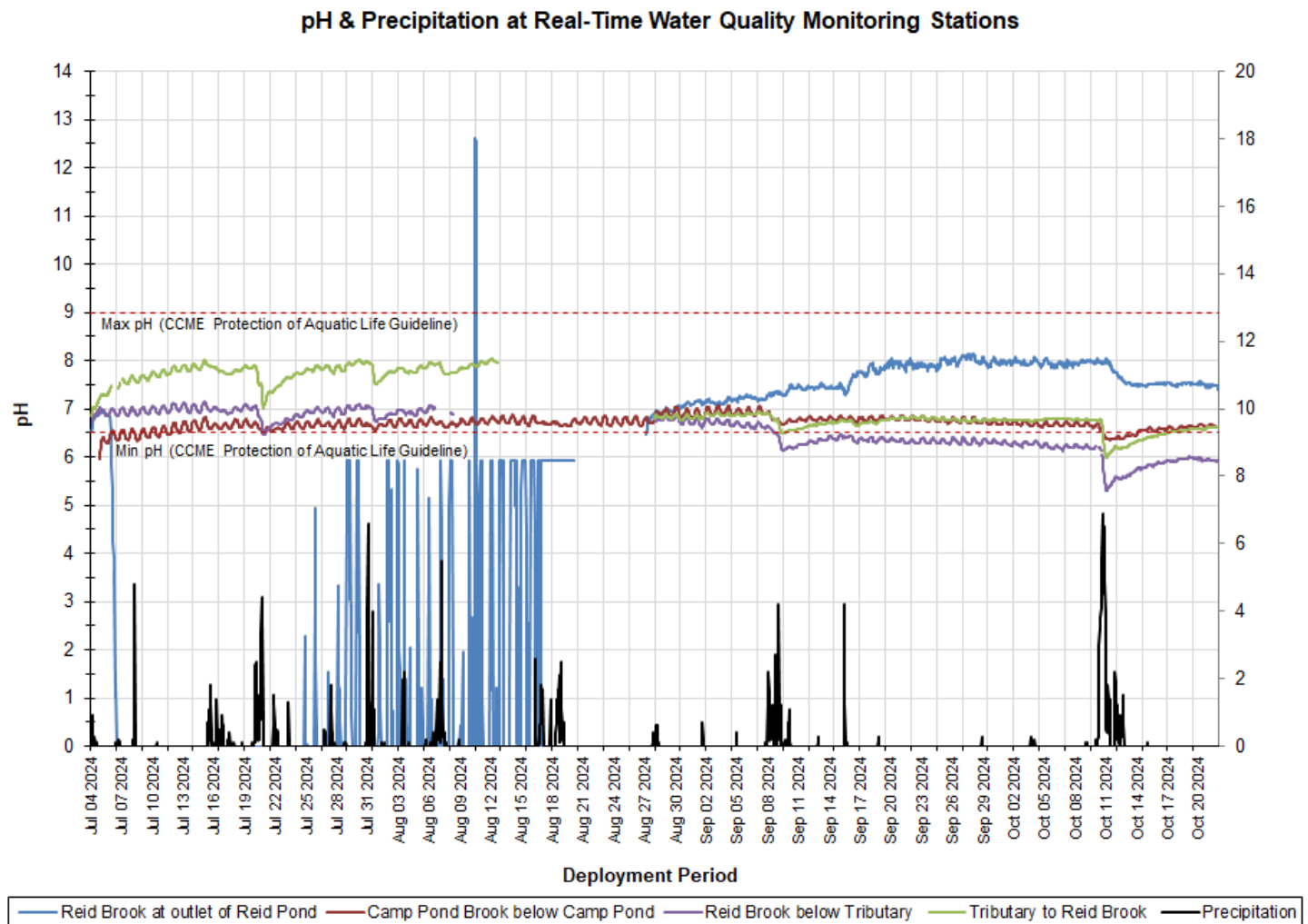
Figure 26: pH & Precipitation at all RTWQ Stations
