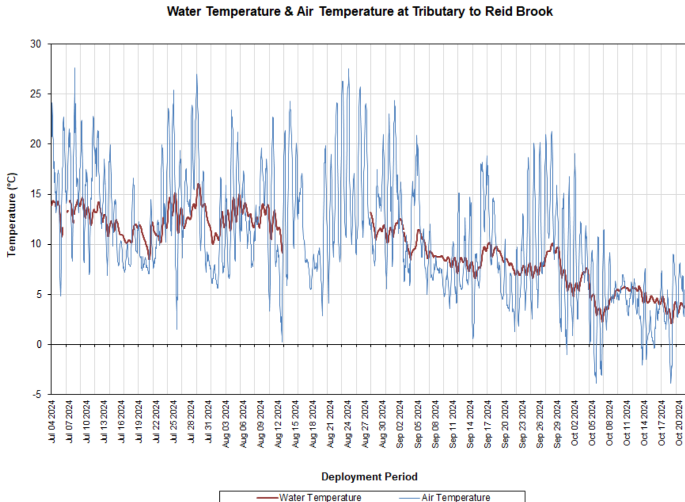
Figure 20: Water Temperature & Air Temperature at Tributary to Reid Brook
