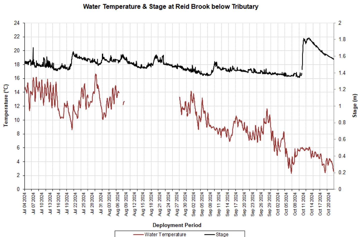
Figure 13: Water Temperature & Stage at Reid Brook below Tributary
