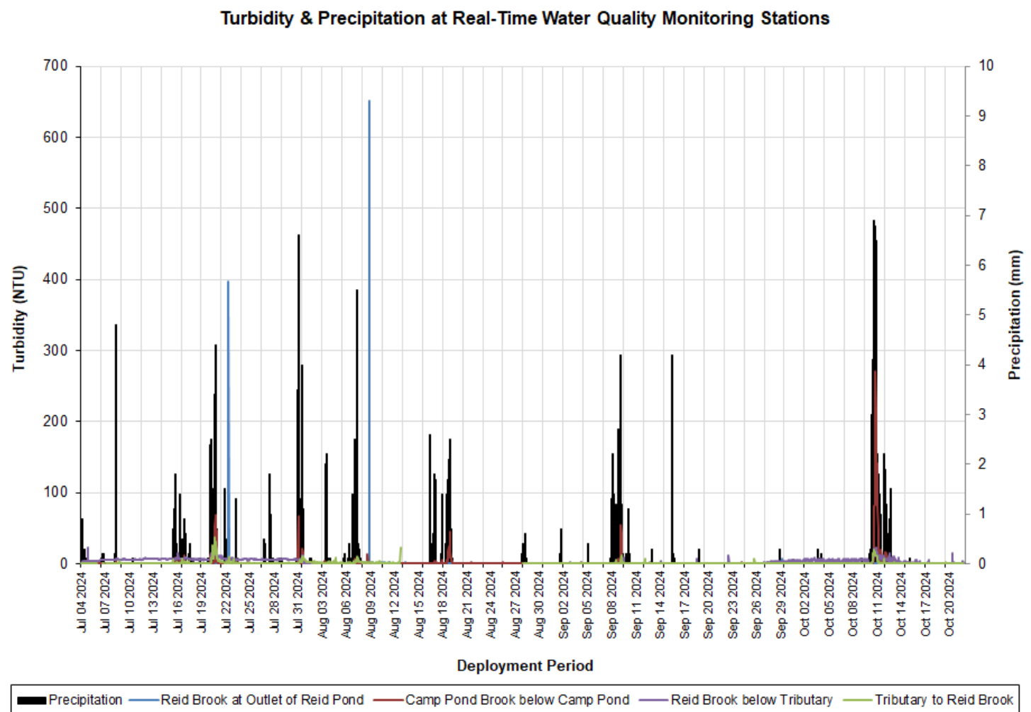
Figure 29a: Turbidity & Precipitation at all RTWQ Stations
