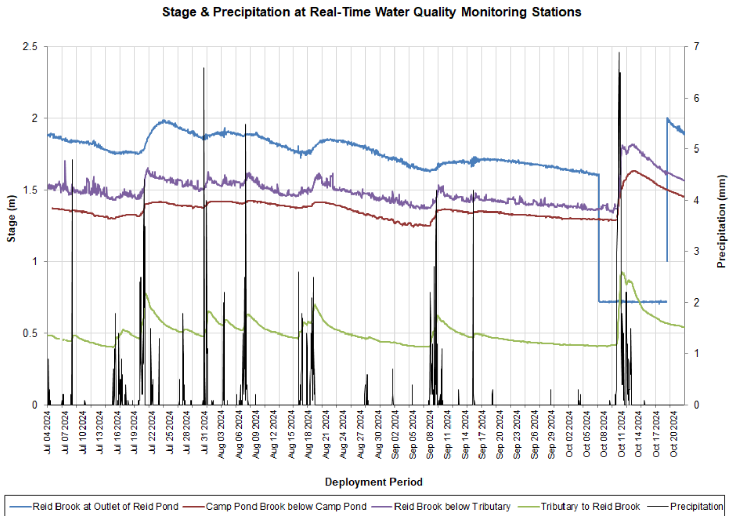
Figure 30: Stage & Precipitation at all RTWQ Stations
