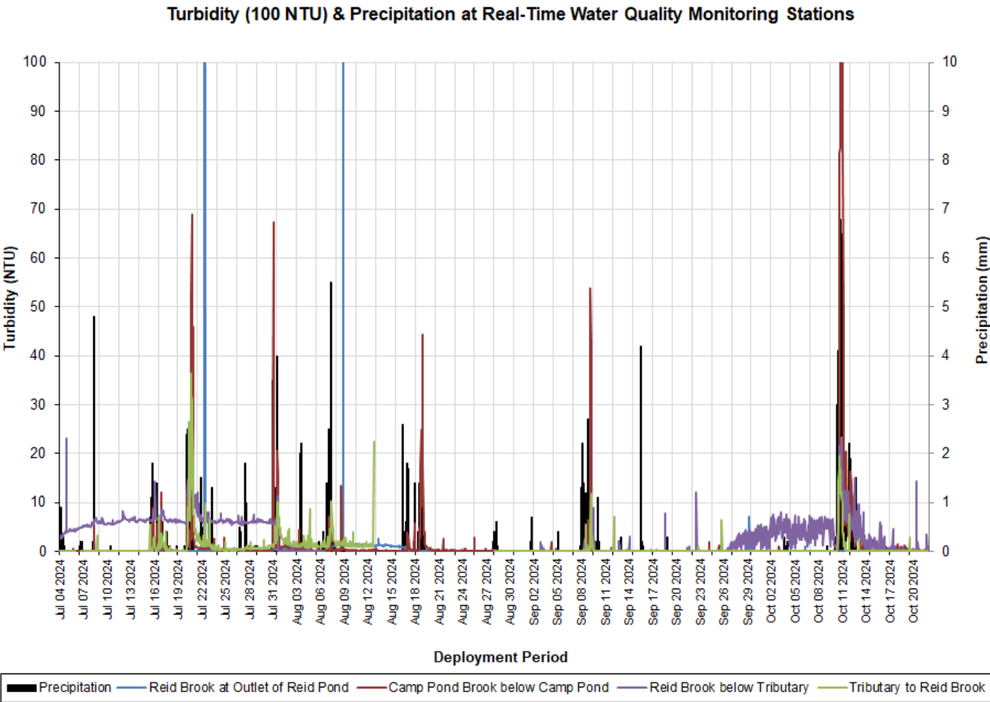
Figure 29b: Turbidity & Precipitation at all RTWQ Stations (graphed to 100 NTU)
