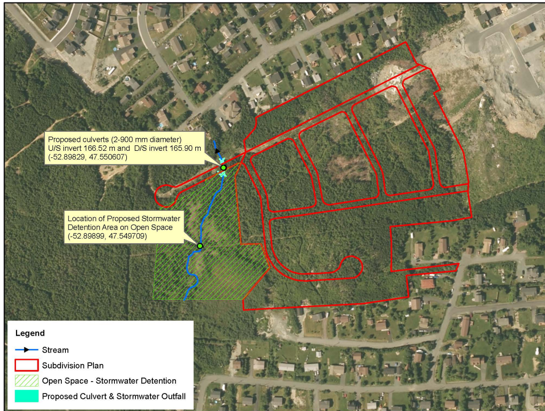
Stormwater Outfall and Culvert Installation at Picco Ridge (Phase 3) Residential Subdivision in Paradise
