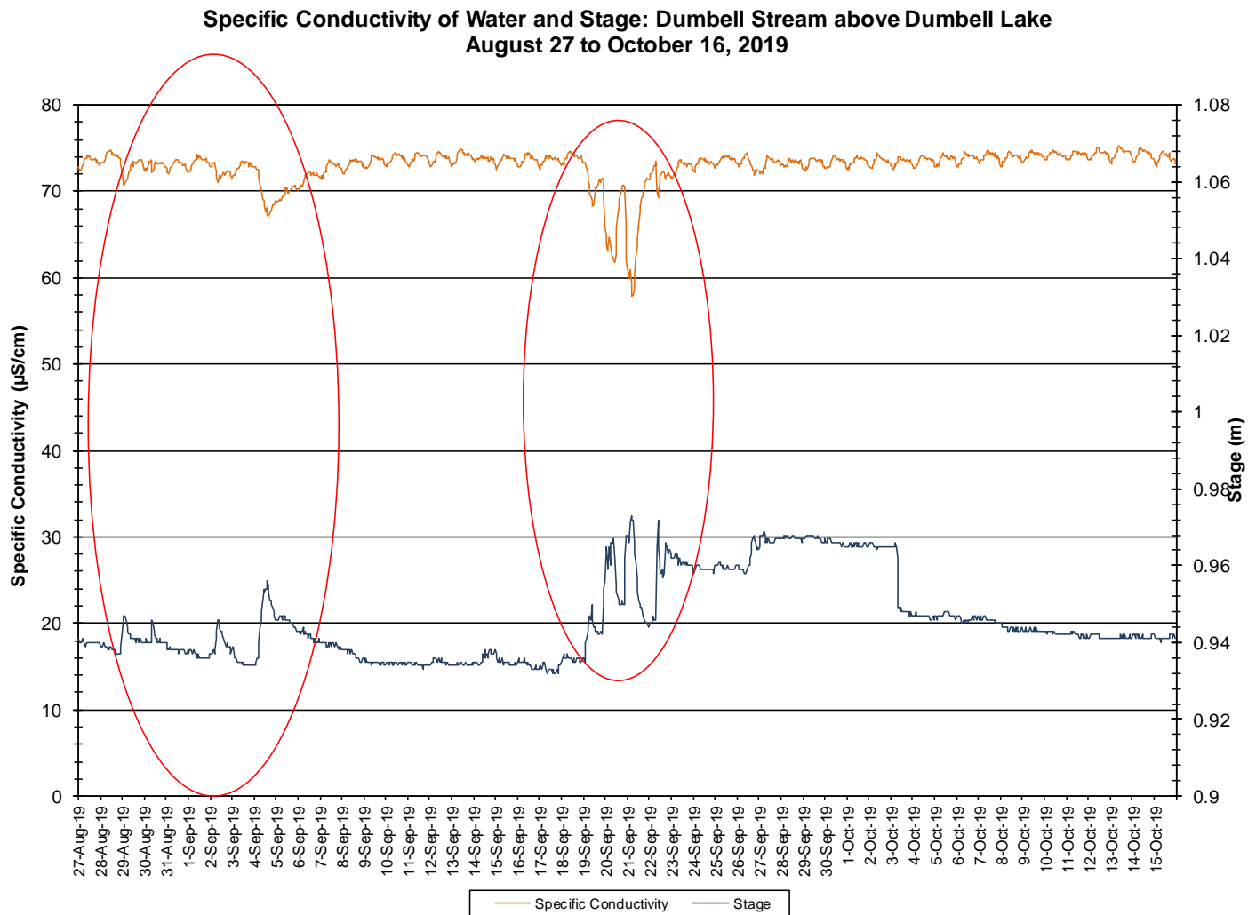
Figure 11: Specific conductivity and stage – Dumbell Stream
