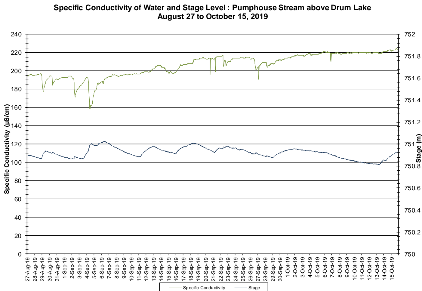
Figure 17: Specific Conductivity and Stage – Pumphouse Stream
