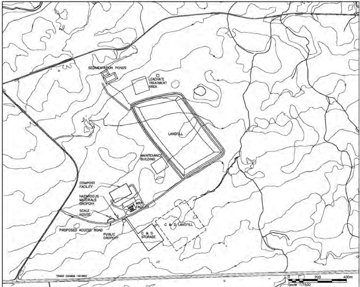
Figure 3: Concept Design of Regional Solid Management Facility for Central Newfoundland.
