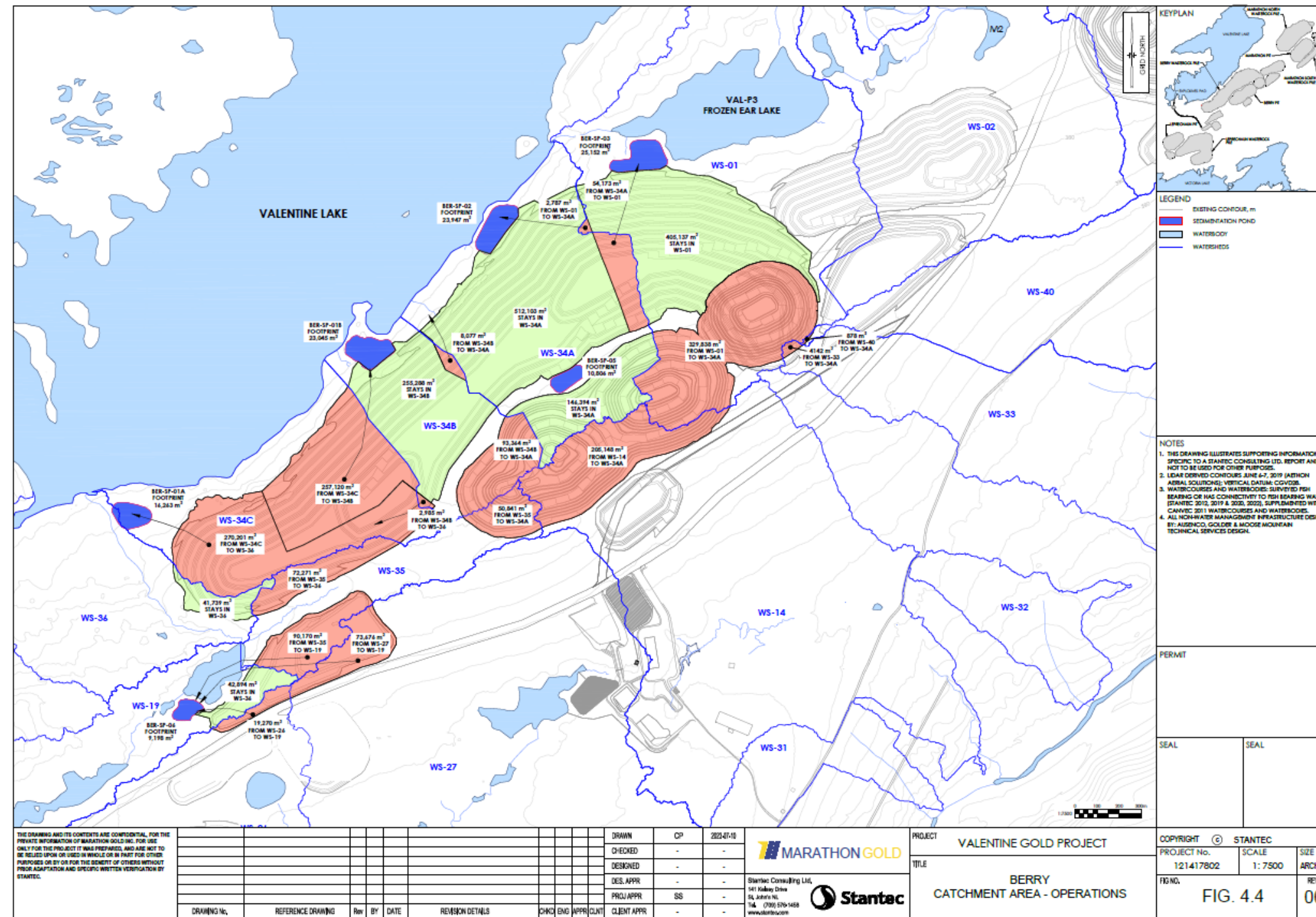
Figure 4.4 Berry Complex Catchment Areas During Operation
