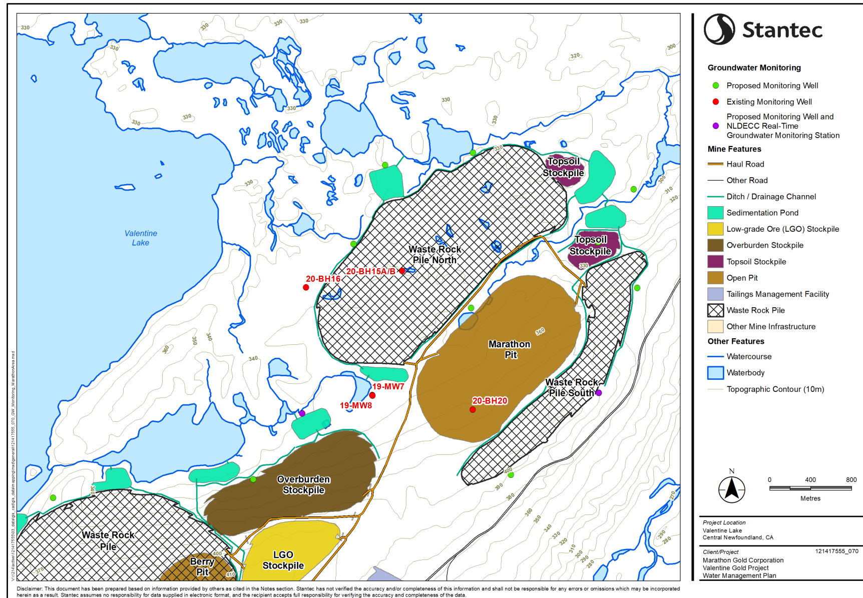
Figure 8.6 Groundwater Monitoring Locations – Marathon Complex
