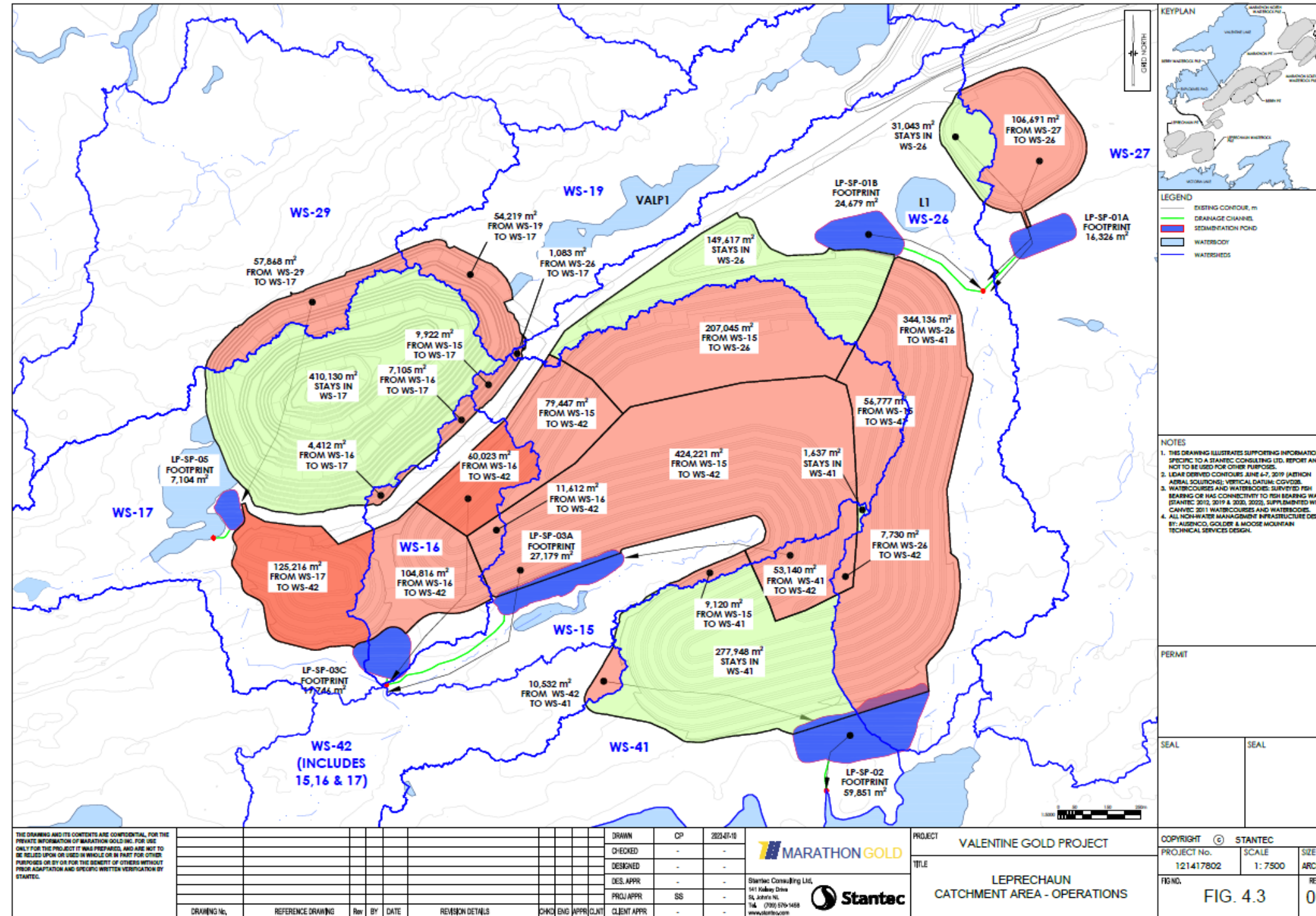
Figure 4.3 Leprechaun Complex Catchment Areas During Operation
