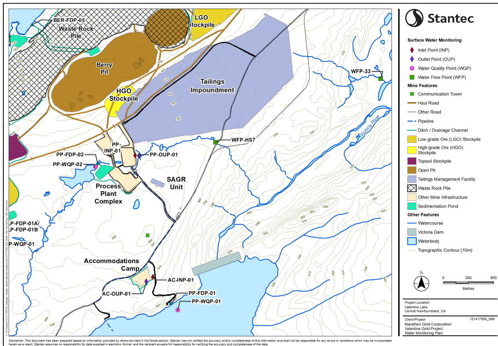
Figure 8.2 Surface Water Monitoring Stations – Processing Plant &amp; TMF Complex
