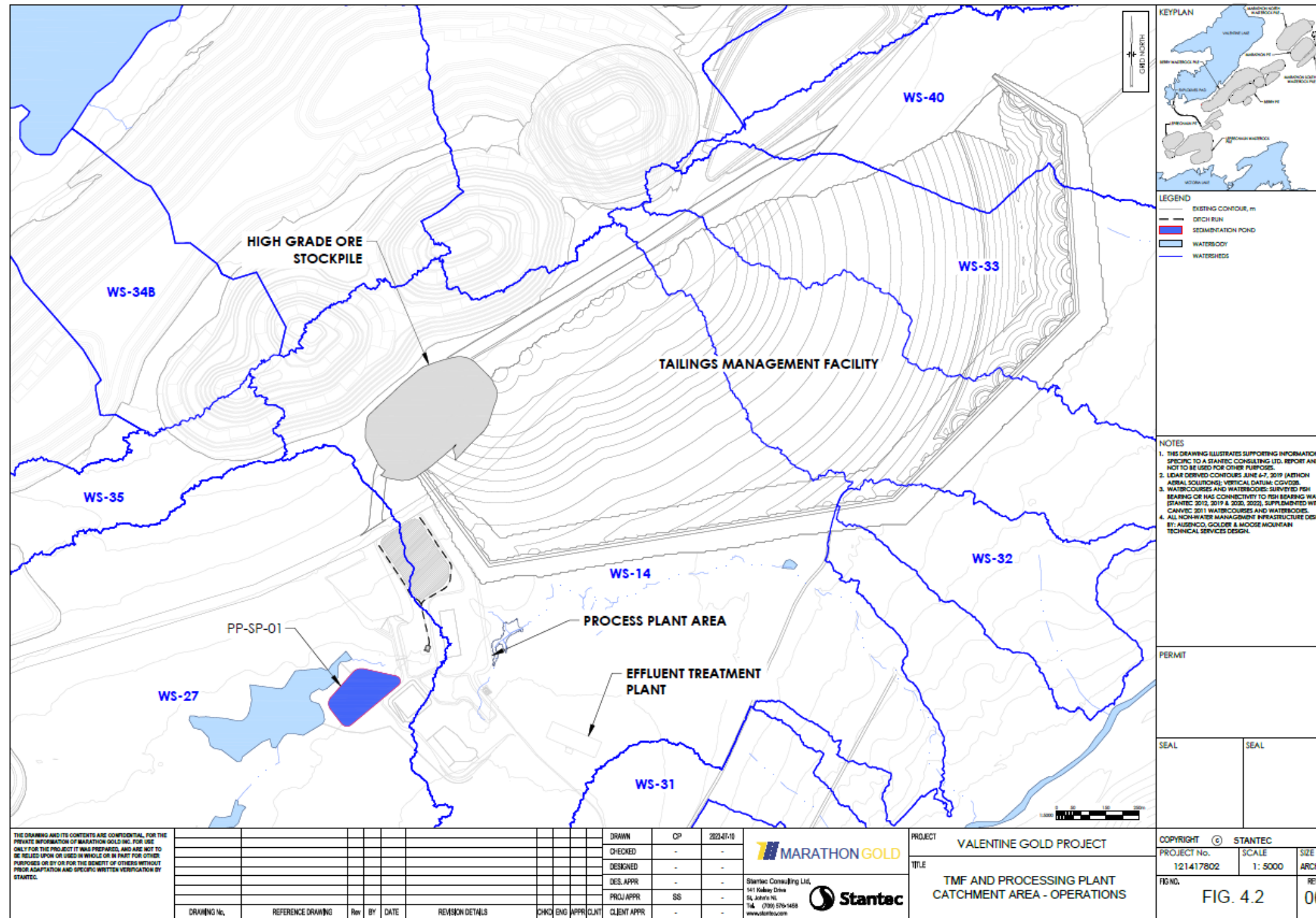
Figure 4.2 Processing Plant and TMF Complex Catchment Areas During Operation
