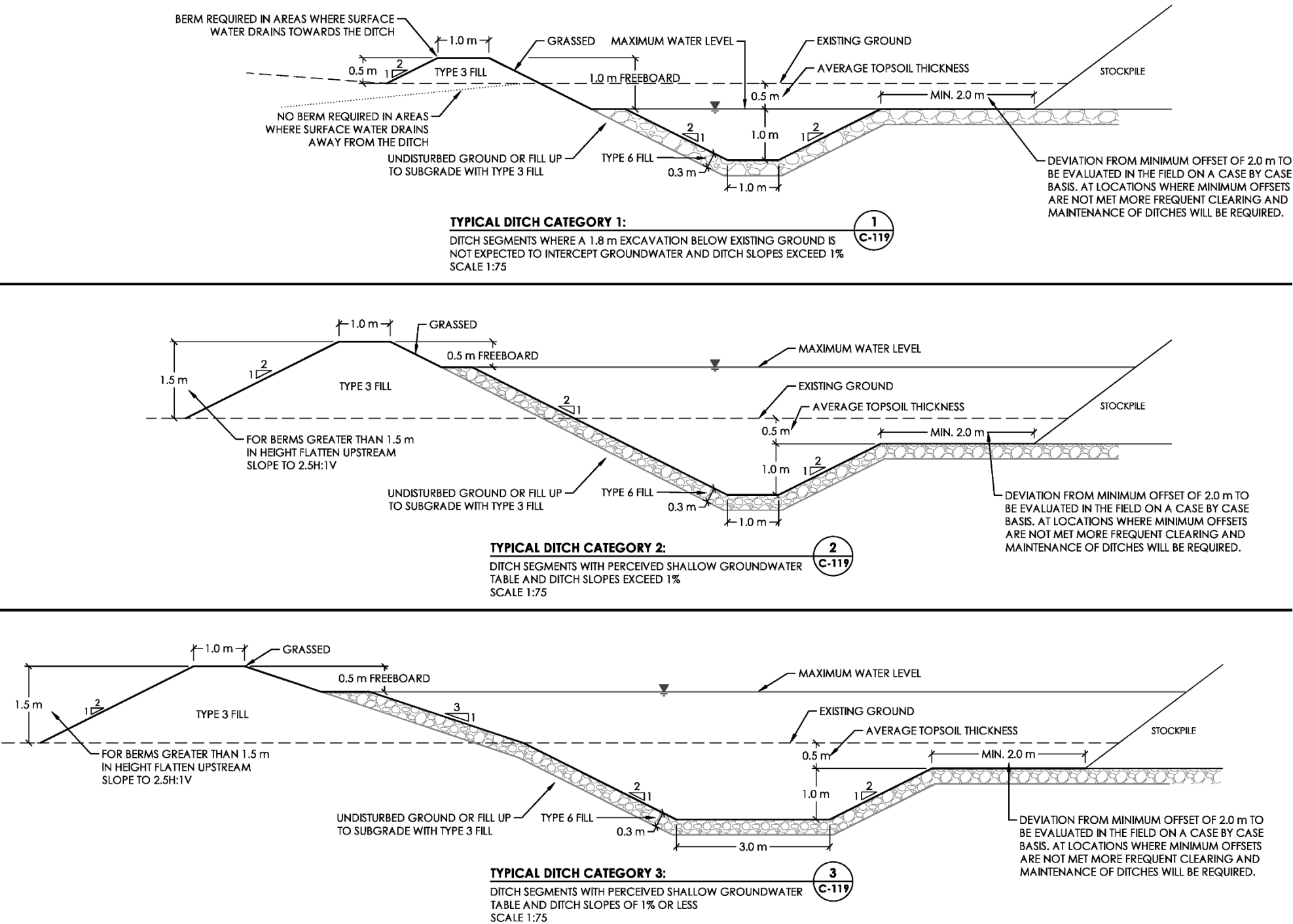
Figure 5.9 Ditch Typical
