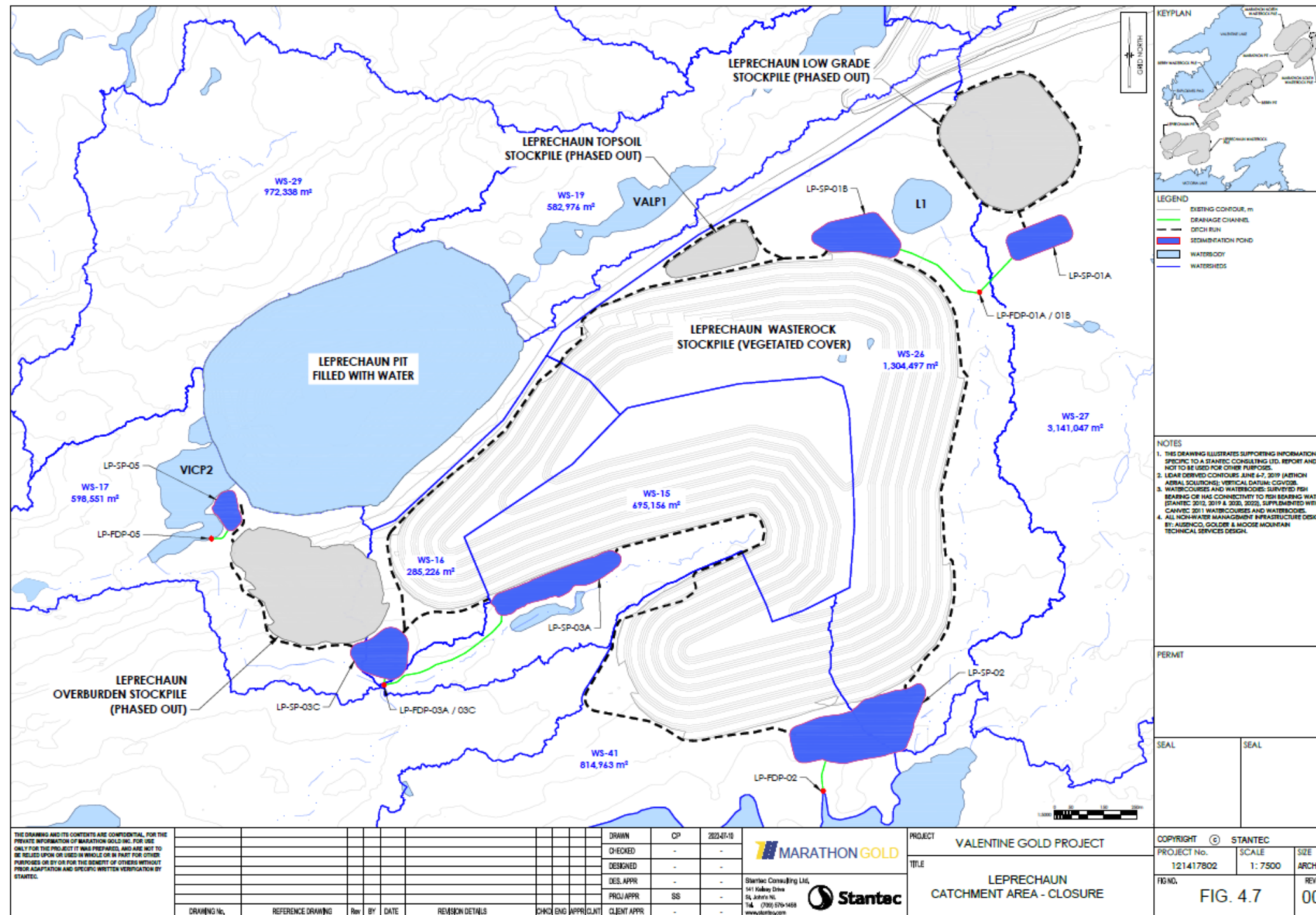
Figure 4.7 Leprechaun Complex Catchment Areas Closure
