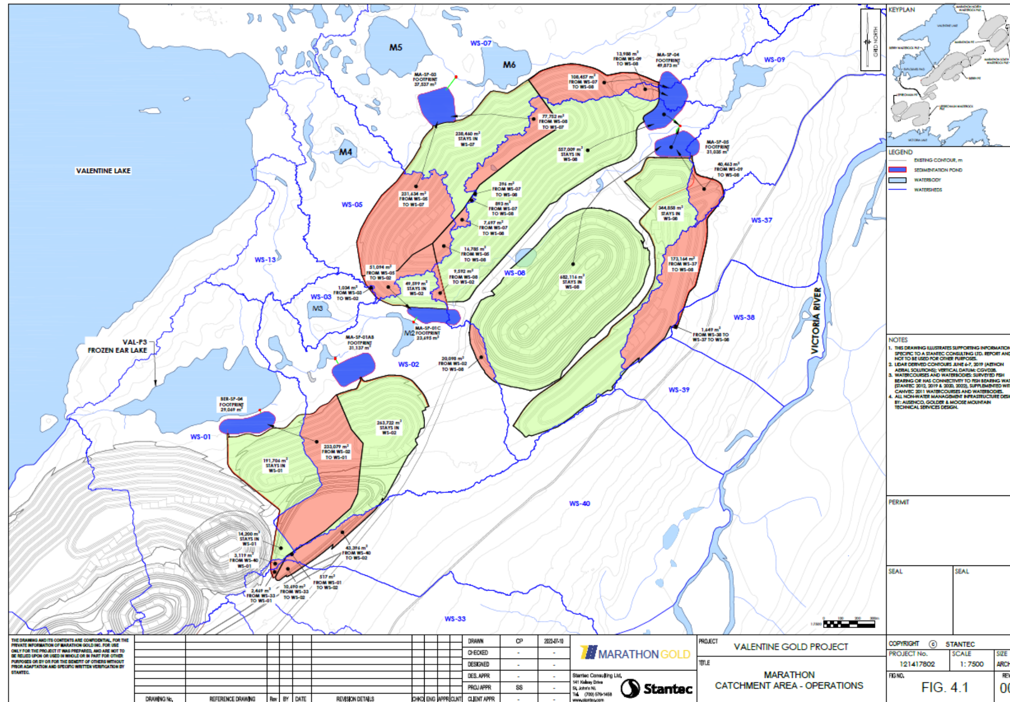
Figure 4.1 Marathon Complex Catchment Areas During Operation
