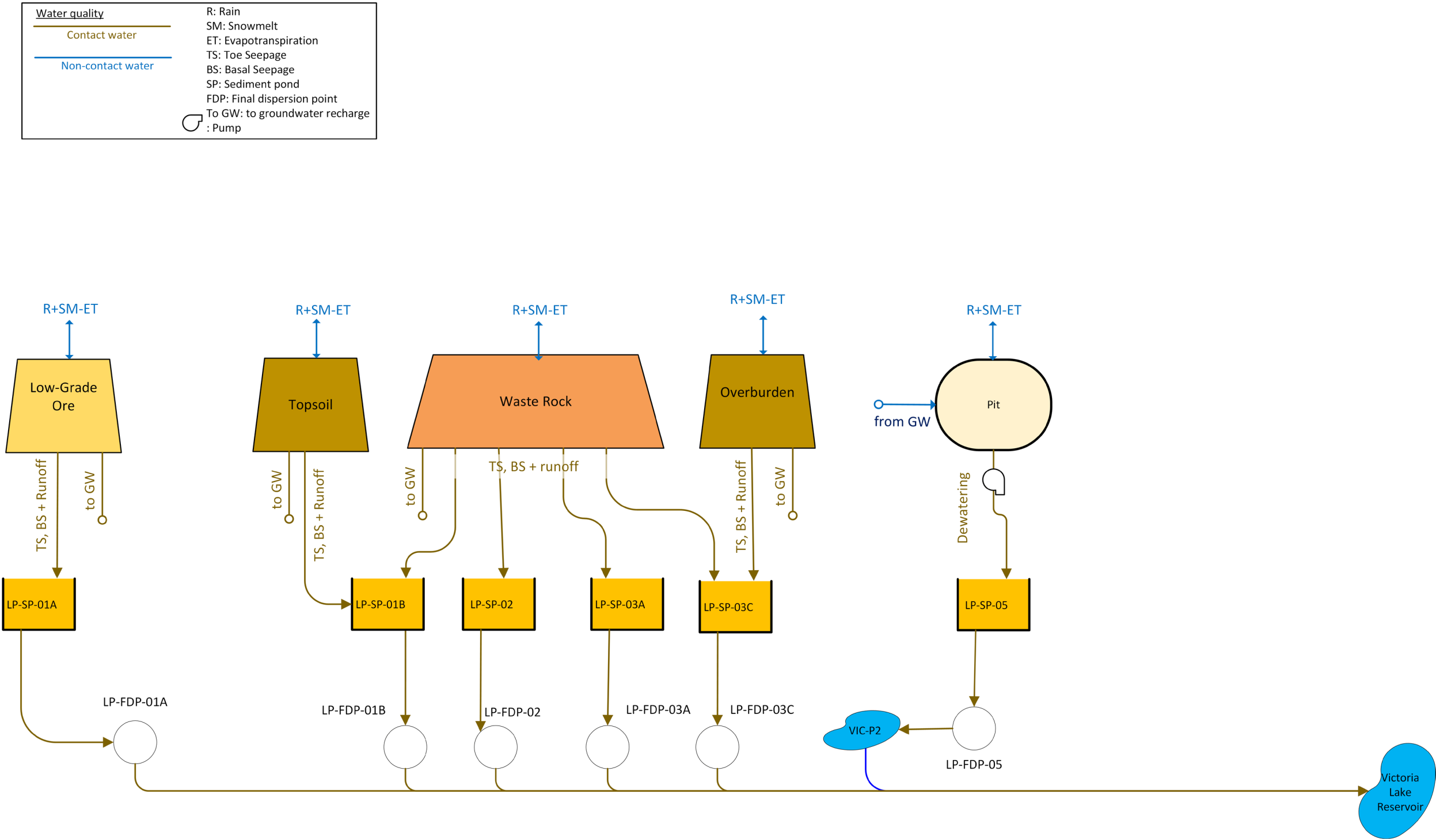
Figure 6.6 Conceptual Model of Mine Water Management – Leprechaun Complex Construction/Operation (Year -1 to 12)
