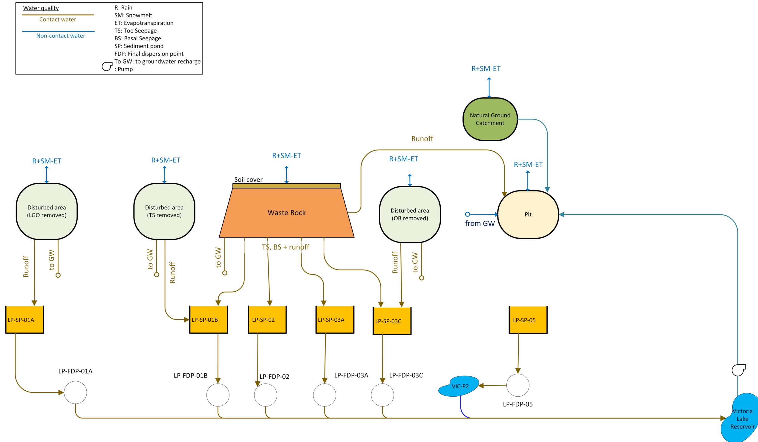
Figure 6.7 Conceptual Model of Mine Water Management – Leprechaun Complex Closure (Year 13 to Pit Full)
