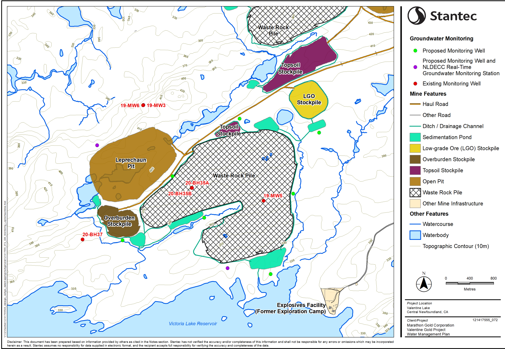
Figure 8.7 Groundwater Monitoring Locations – Leprechaun Complex
