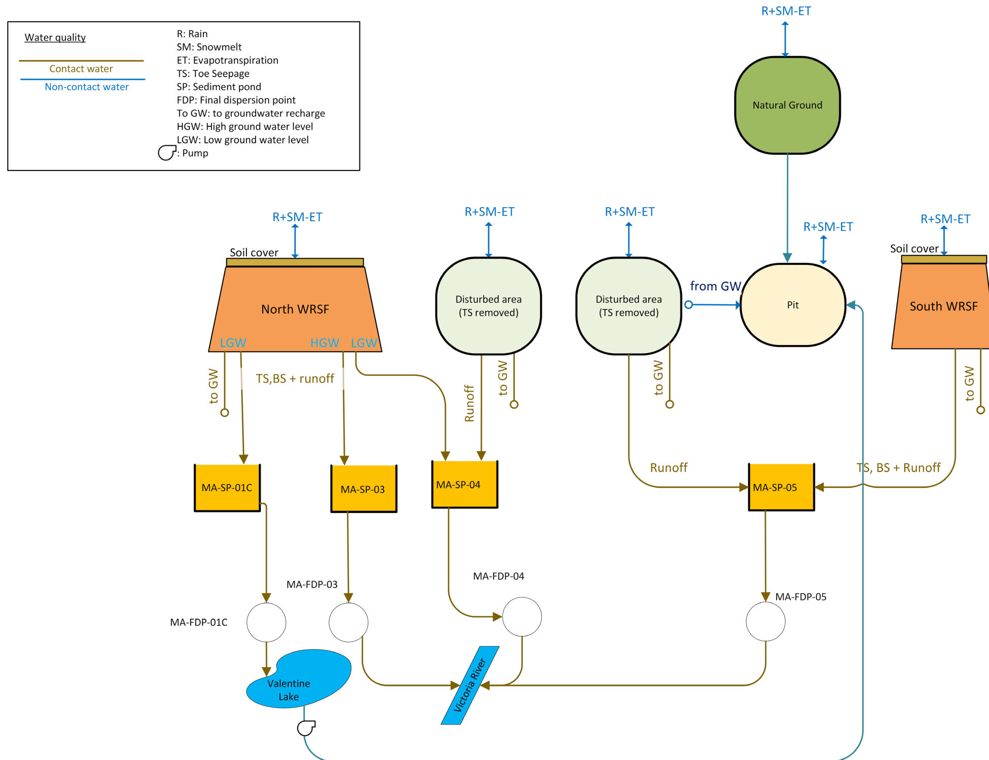
Figure 6.4 Conceptual Model of Mine Water Management – Marathon Complex Closure (Year 14 until Pit is full)
