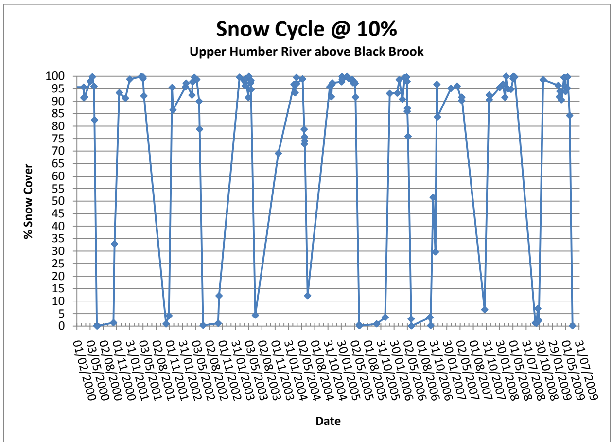
Plot of Snow Cover Data with 10% Cloud Cover Threshold
