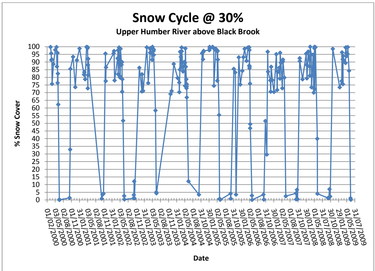
Plot of Snow Cover Data with 30% Cloud Cover Threshold
