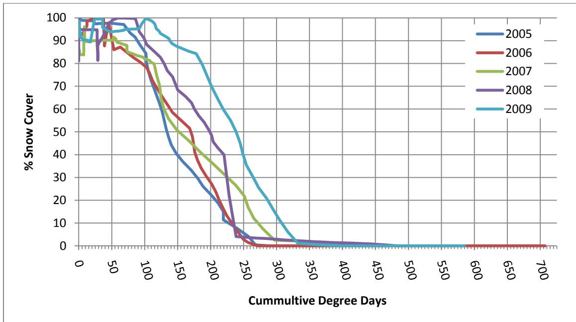
‘Type II Curves from 2005 to 2009’
