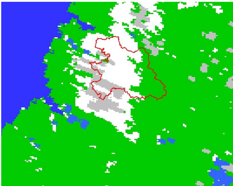
Figure 2.3: Processed MODIS/Terra Snow Covered Area for the Upper Humber Basin, NL
