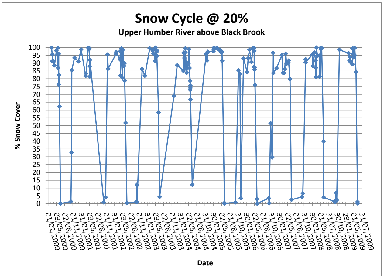
Plot of Snow Cover Data with 20% Cloud Cover Threshold
