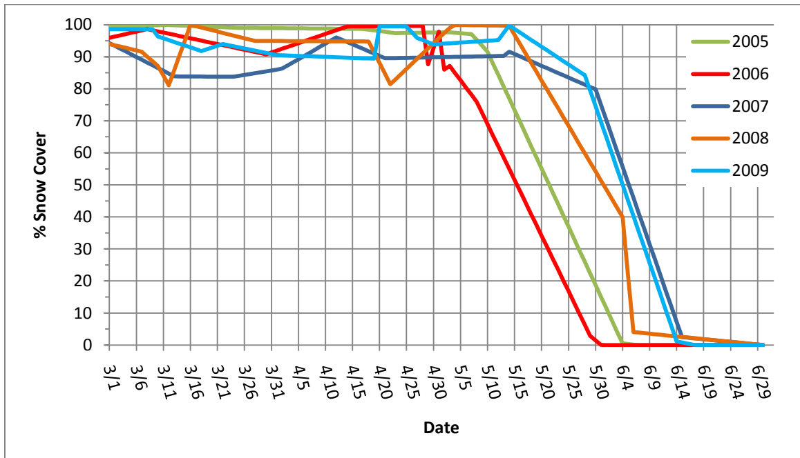
‘Type I Curves from 2005 to 2009’
