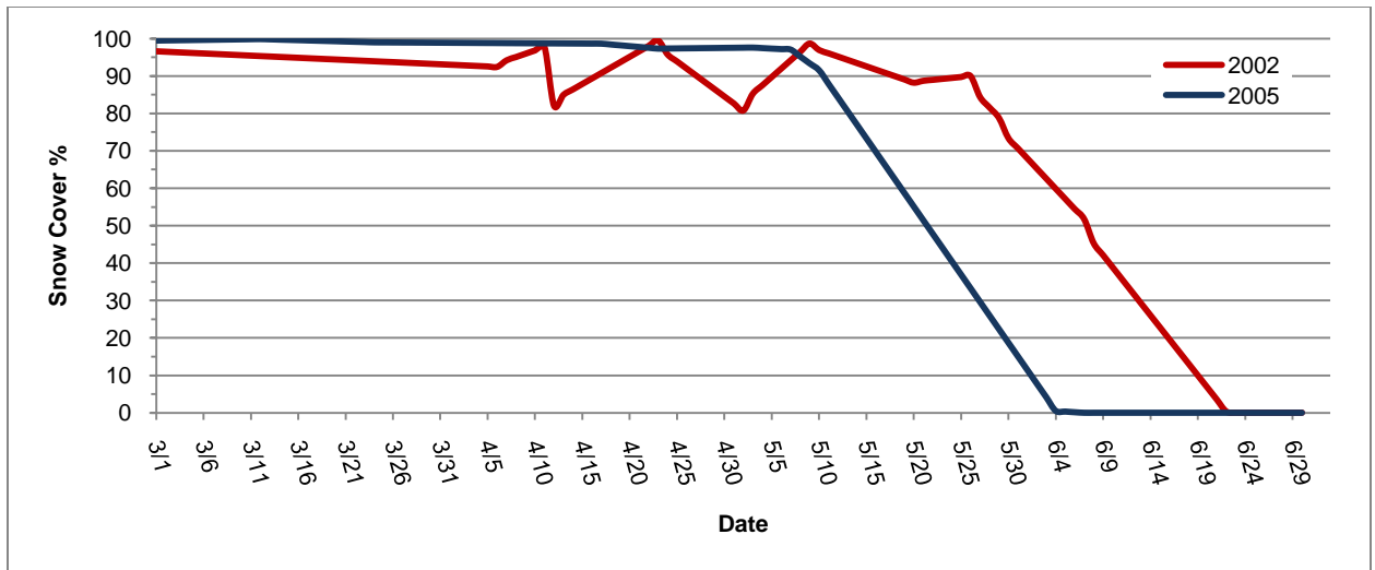
Figure 2.5: Typical Type I Conventional Snow Depletion Curves at 20% Cloud Cover
