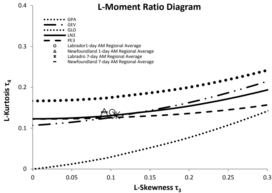
Figure 4-2 L-moment ratio diagram and regional averages
