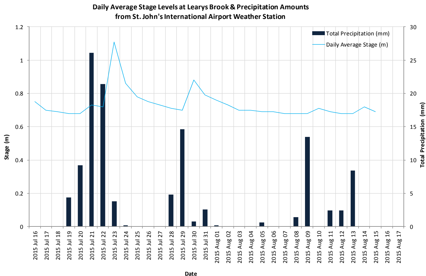
Figure 7: Daily average stage values (m) from Leary's Brook Station and daily total precipitation values (mm) from St. John's International Airport.
