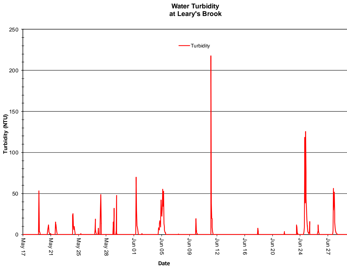
Figure 6: Turbidity (NTU) values at Leary's Brook Station
