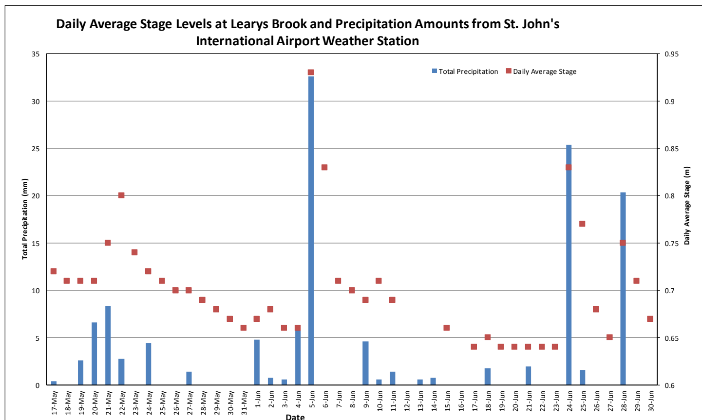
Figure 7: Daily average stage values (m) from Leary's Brook Station and daily total precipitation values (mm) from St. John's International Airport.
