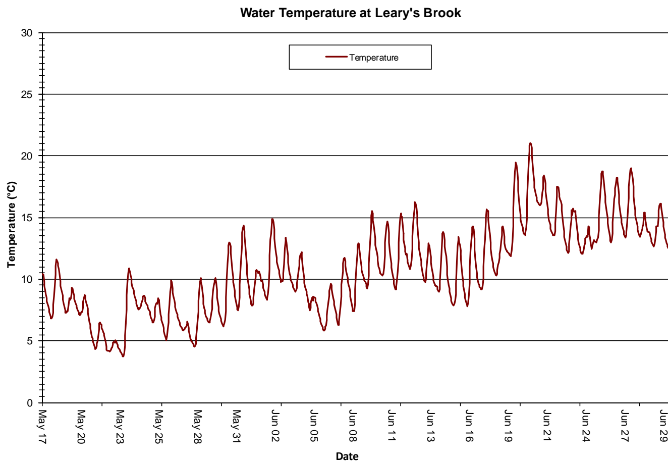
Figure 2: Water Temperature at Leary's Brook
