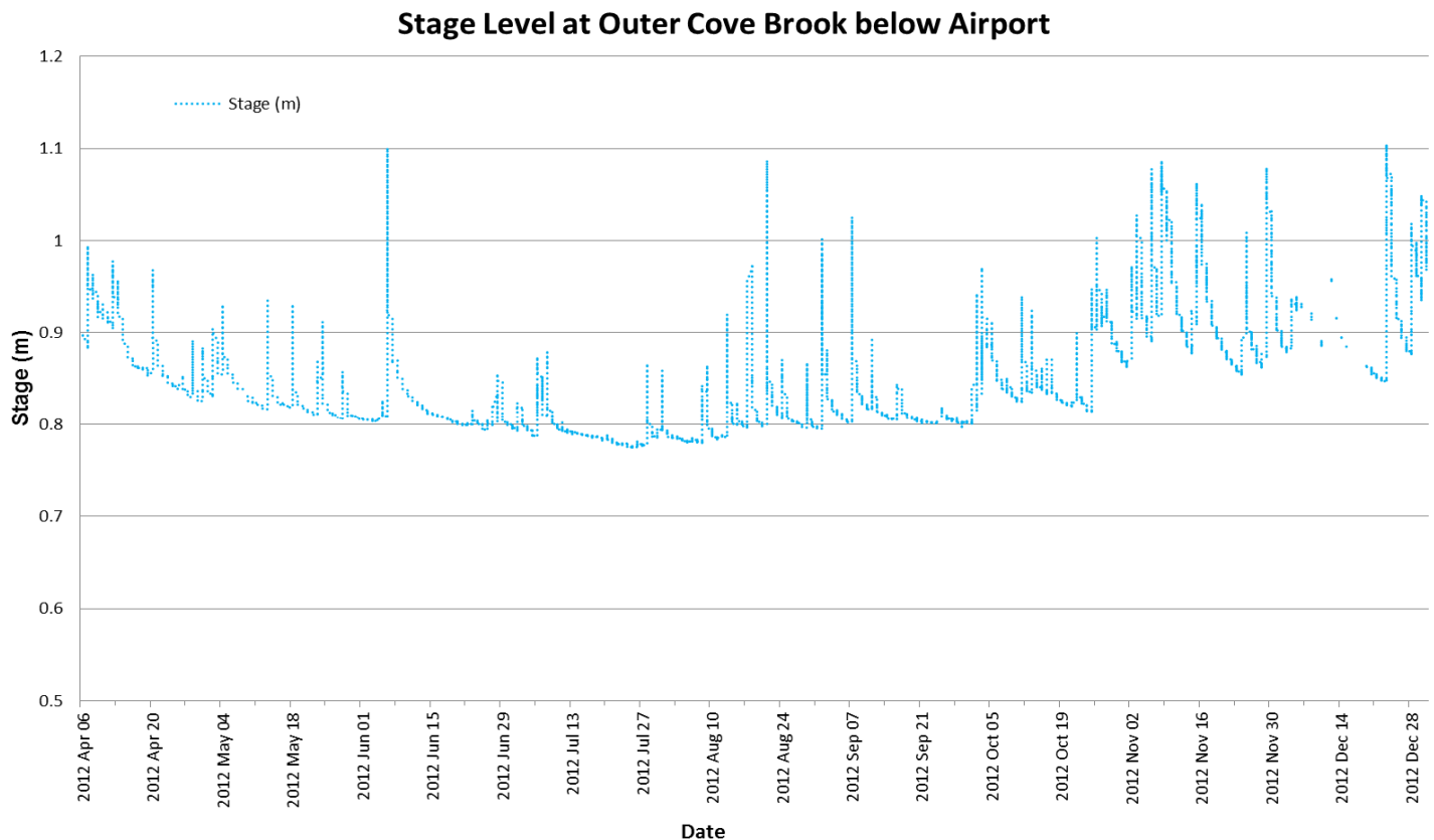
Figure 5: Quarter-hourly stage (m) values recorded at Outer Cove Brook below Airport from April 6 to December 31, 2012.
