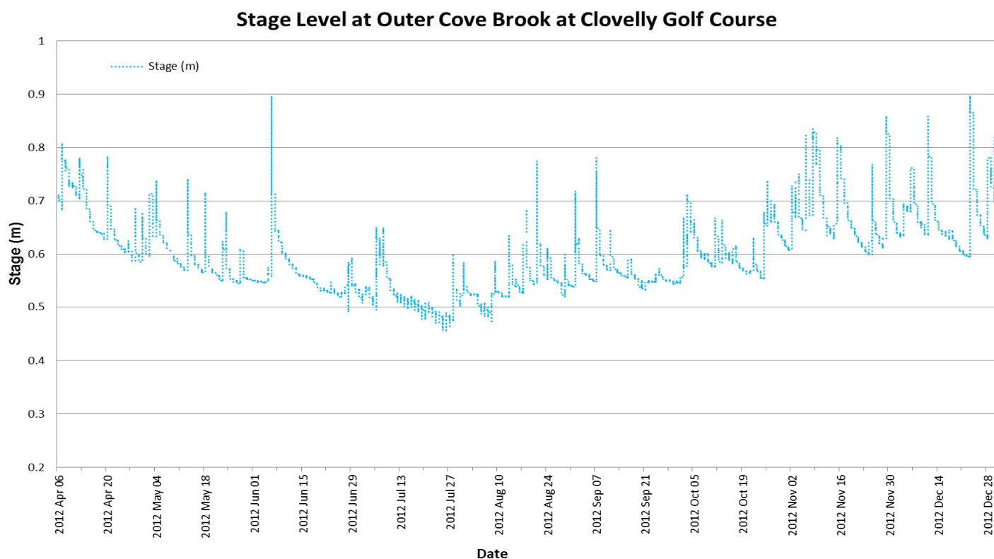
Figure 11: Quarter-hourly stage (m) values recorded at Outer Cove Brook at Clovelly Golf Course from April 6 to December 31, 2012.
