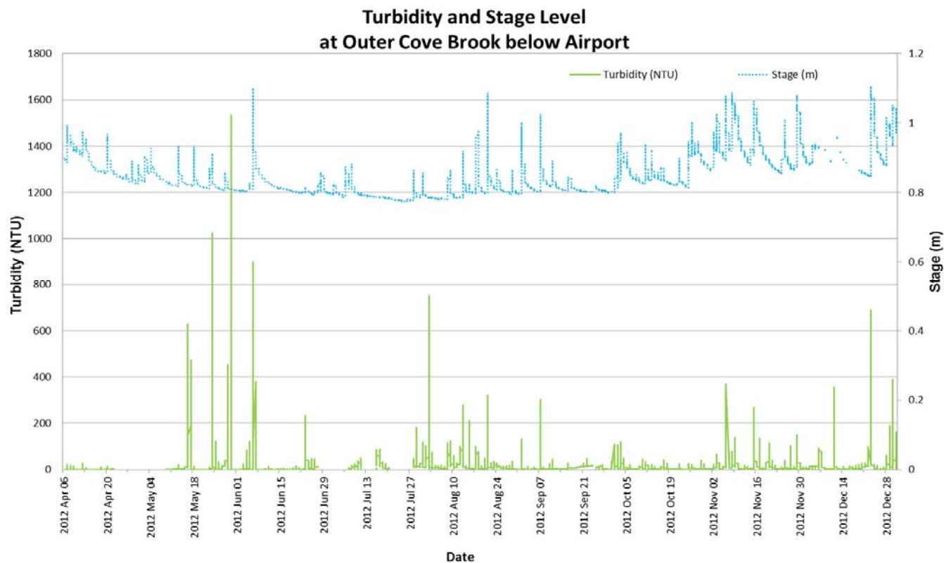
Figure 9: Quarter-hourly turbidity (NTU) and stage level (m) values recorded at Outer Cove Brook below Airport from April 6 to December 31, 2012.
