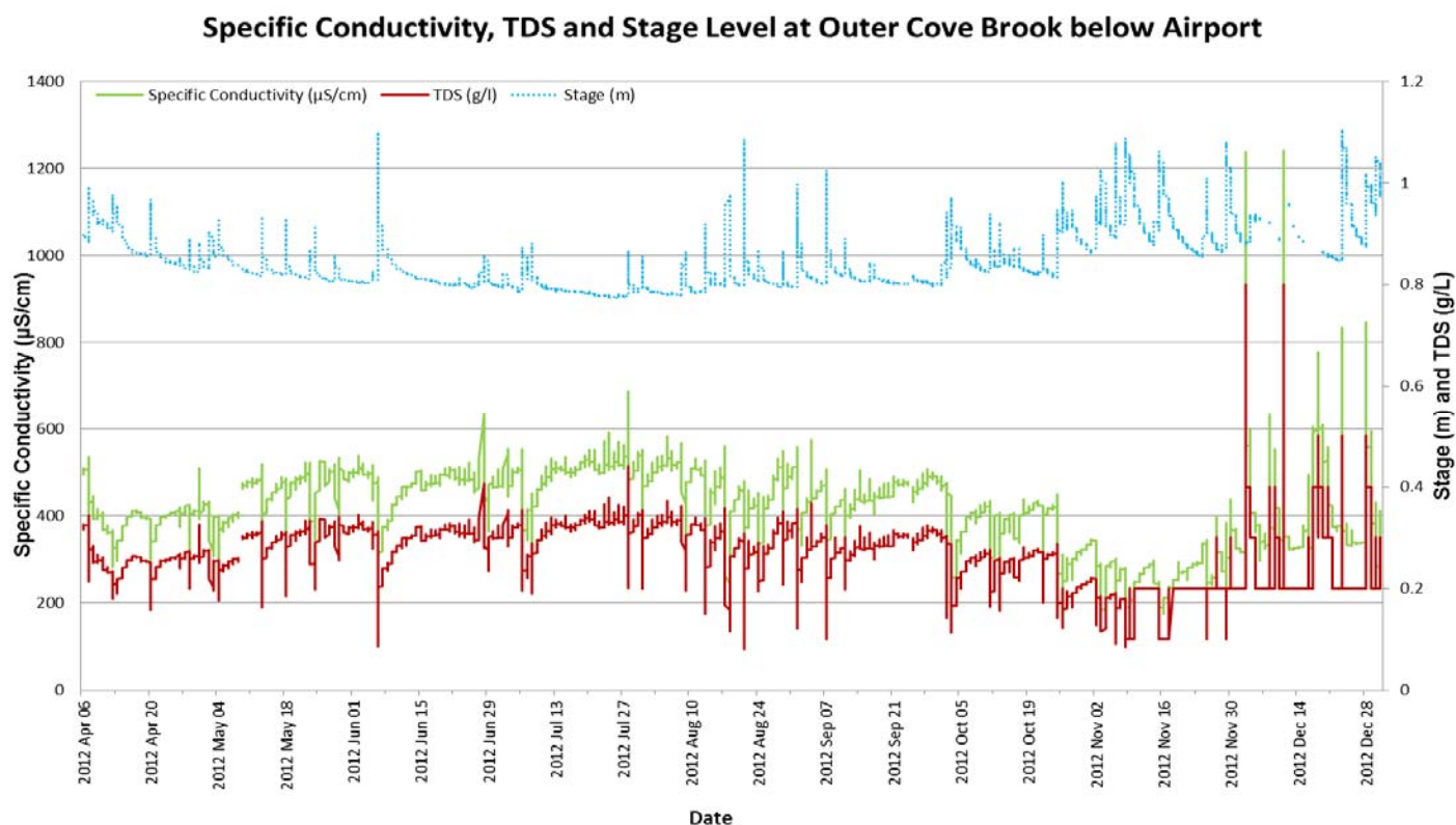
Figure 8: Quarter-hourly specific conductivity ( \mu\text{S}/\text{cm} ), total dissolved solids (g/L) and stage level (m) values recorded at Outer Cove Brook below Airport from April 6 to December 31, 2012.
