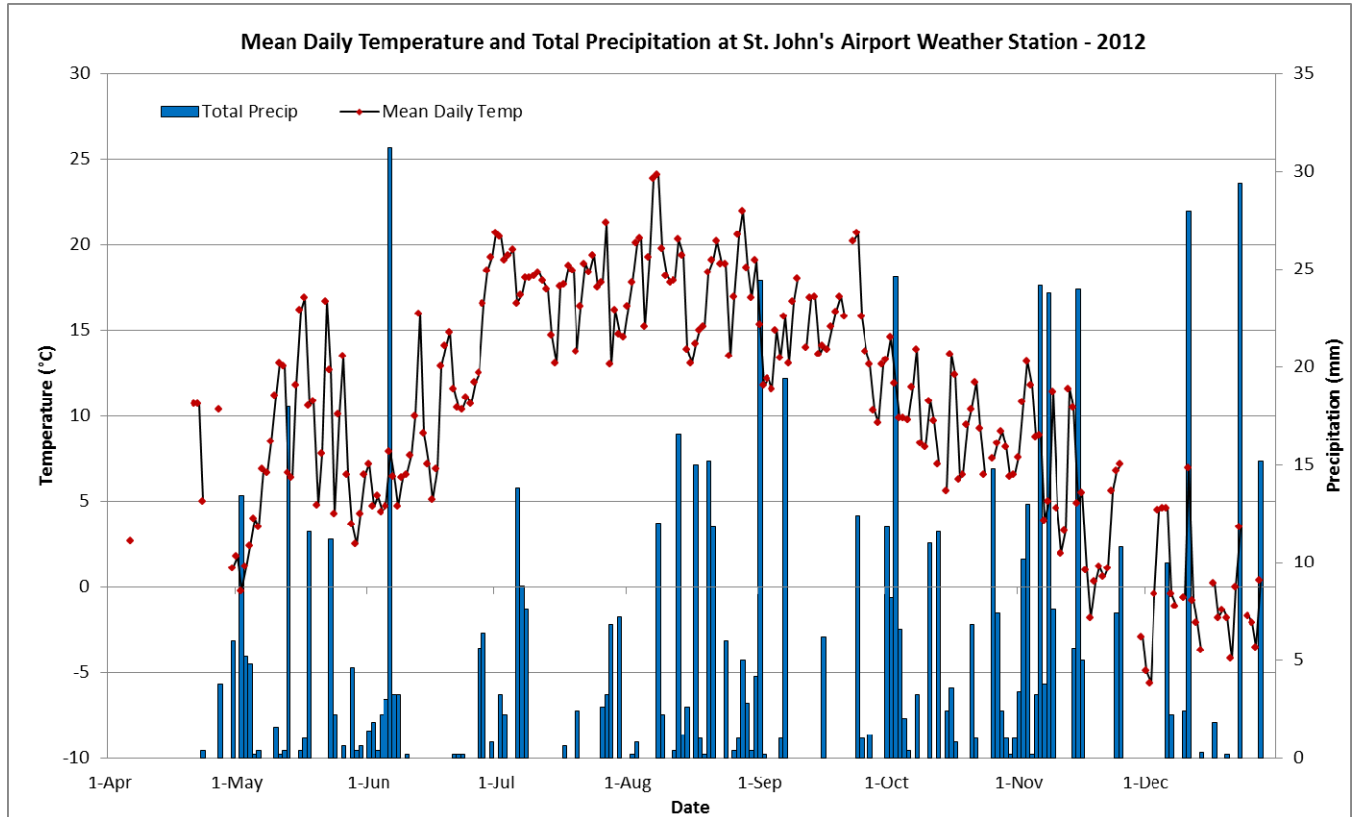
Figure 17: Mean daily temperature and total precipitation values for the period April 1 to December 31, 2012, from Environment Canada's St. John's International Airport weather station.
