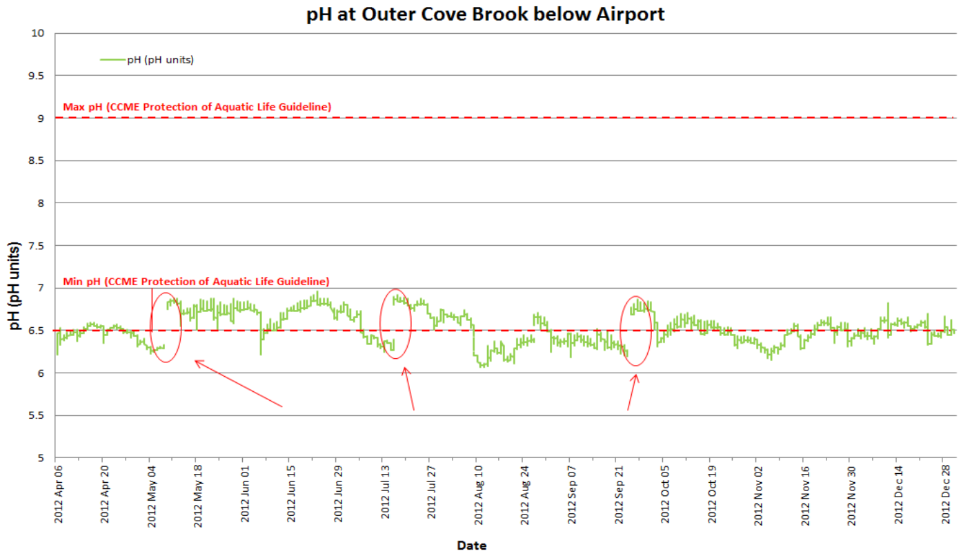
Figure 7: Quarter-hourly pH (pH units) values recorded at Outer Cove Brook below Airport from April 6 to December 31, 2012.
