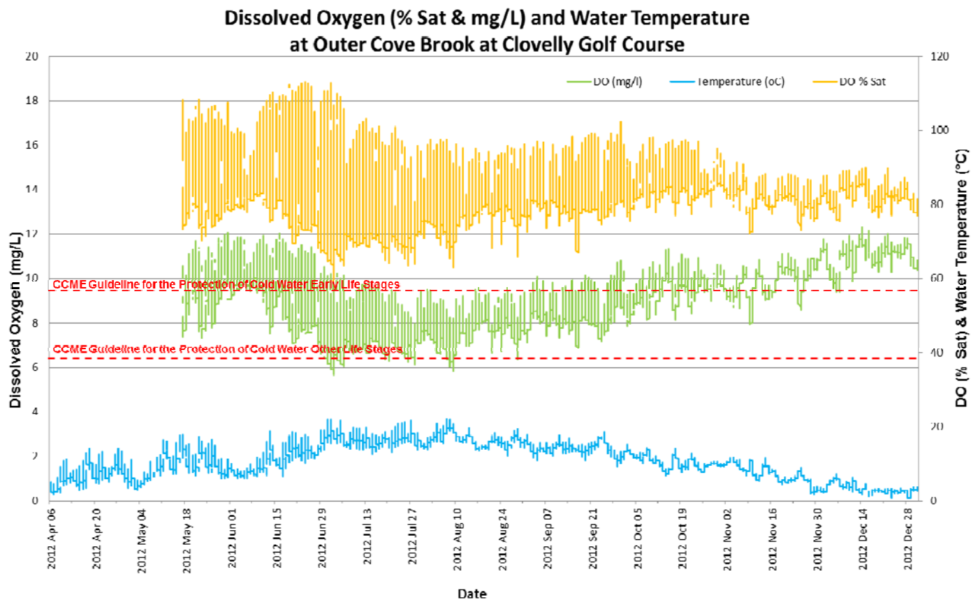
Figure 16: Quarter-hourly dissolved oxygen (% Sat & mg/L) and water temperature (°C) values recorded at Outer Cove Brook at Clovelly Golf Course from April 6 to December 31, 2012
