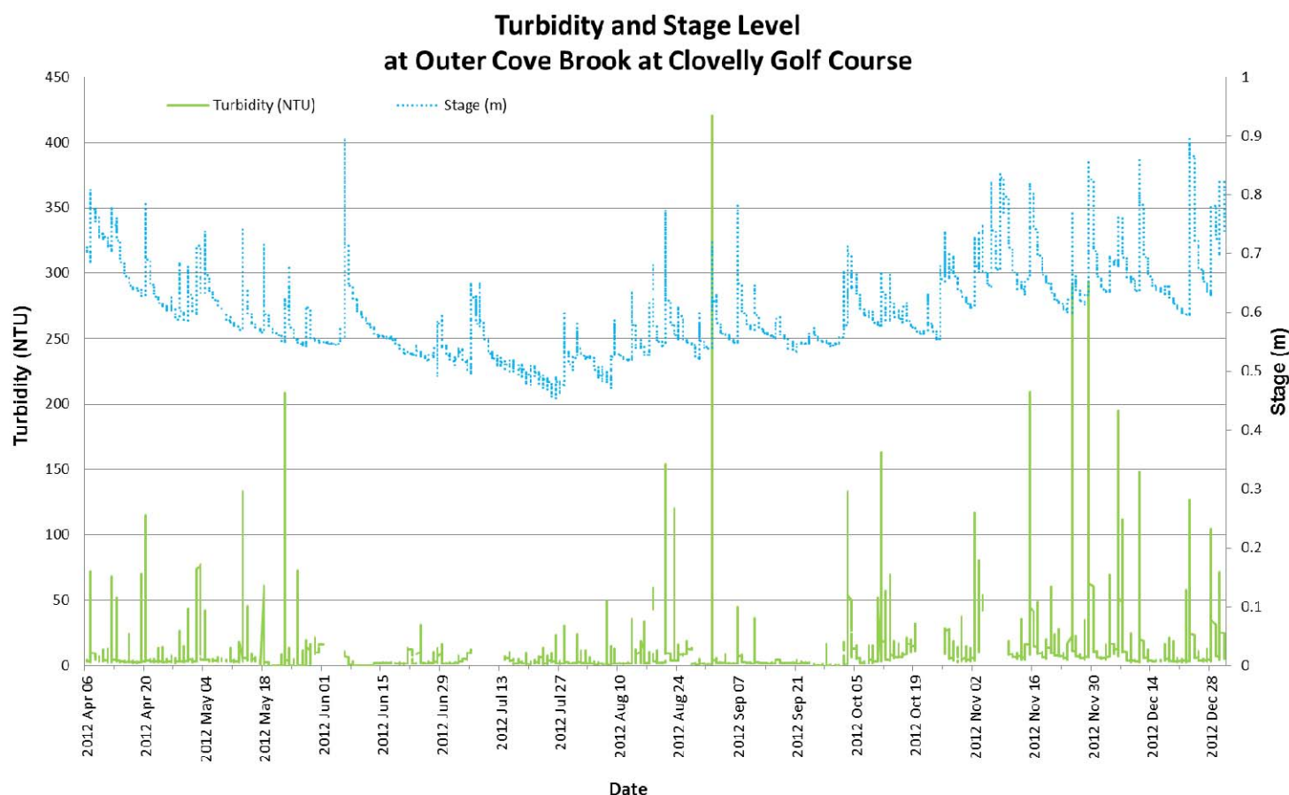
Figure 15: Quarter-hourly turbidity (NTU) and stage level (m) values recorded at Outer Cove Brook at Clovelly Golf Course from April 6 to December 31, 2012.
