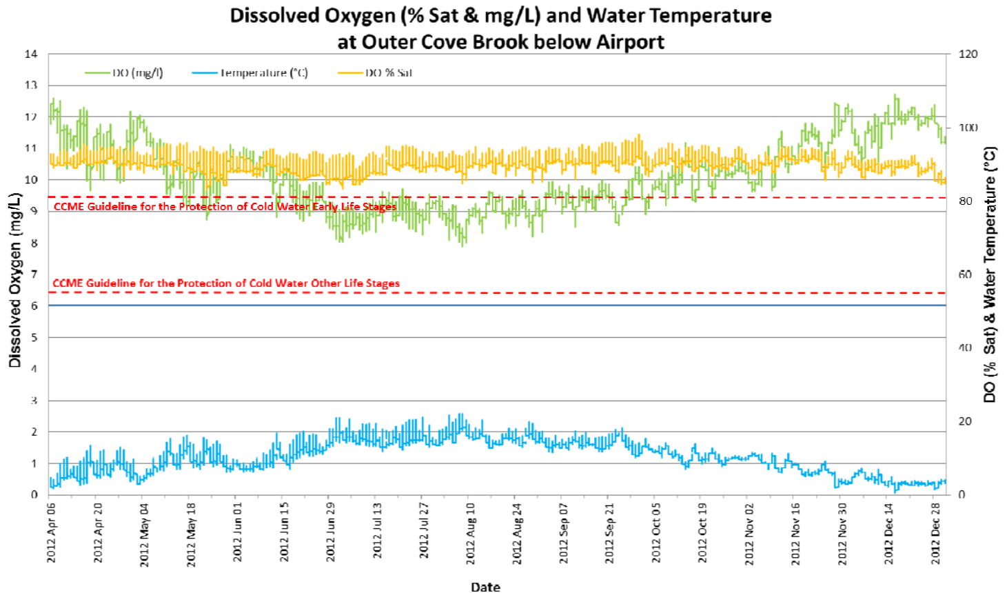
Figure 10: Quarter-hourly dissolved oxygen (% Sat & mg/L) and water temperature (°C) values recorded at Outer Cove Brook below Airport from April 6 to December 31, 2012
