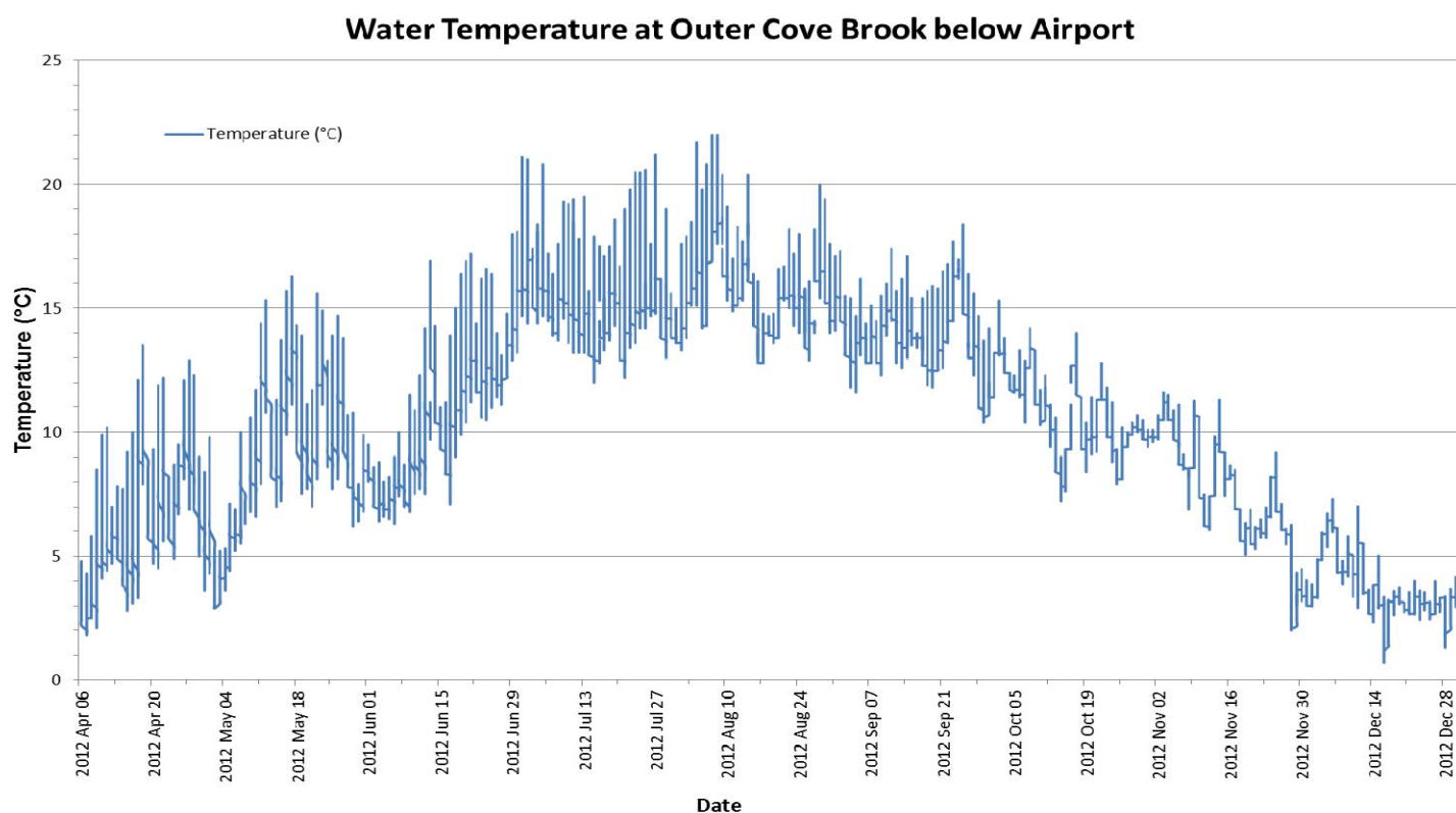
Figure 6: Quarter-hourly temperature (°C) values recorded at Outer Cove Brook below Airport from April 6 to December 31, 2012.
