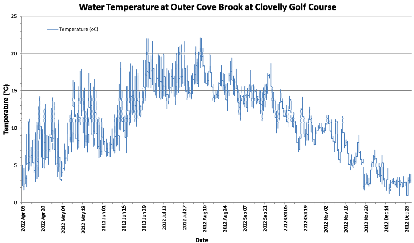
Figure 12: Quarter-hourly temperature (°C) values recorded at Outer Cove Brook at Clovelly Golf Course from April 6 to December 31, 2012.
