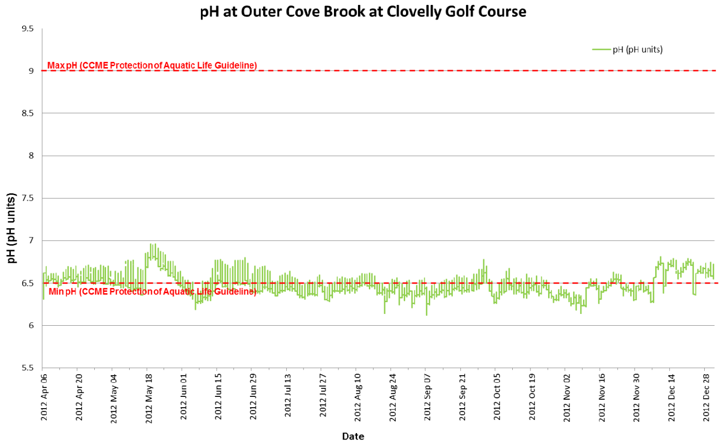
Figure 13: Quarter-hourly pH (pH units) values recorded at Outer Cove Brook at Clovelly Golf Course from April 6 to December 31, 2012.
