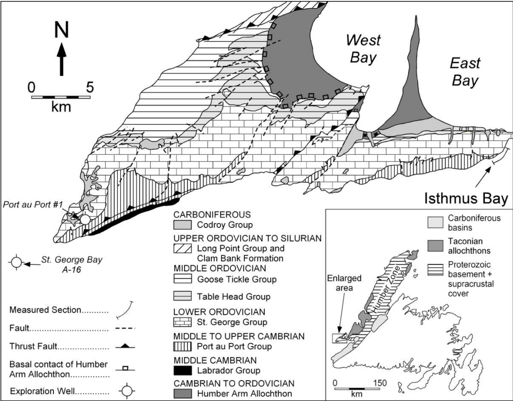
Figure 1: Geological map of the Port au Port peninsula showing locating of the Isthmus Bay section (modified from Knight et al. 2008).
