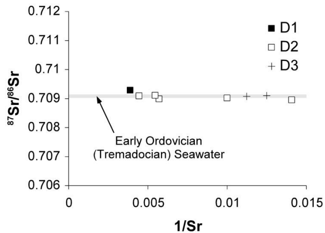
Figure 8: Scatter diagram showing the ^{87}\text{Sr}/^{86}\text{Sr} values in the Watts Bight dolomites (D1 to D3). The shaded area represents the range of ^{87}\text{Sr}/^{86}\text{Sr} values for the Tremadoc (Veizer et al. 1999; Shields et al. 2003)
