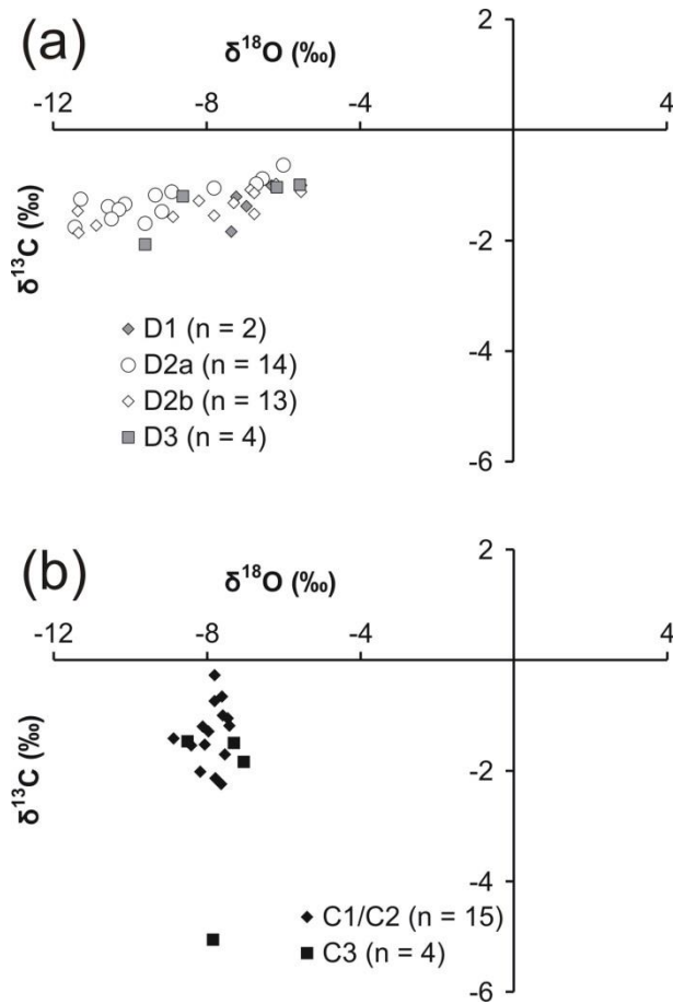
Figure 7: Oxygen vs. Carbon isotope values for (a) dolomite (D1, D2a, D2b, D3) and (b) calcite (C1/C2, C3).
