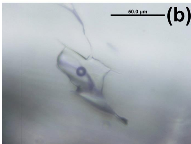
Figure 4: Photomicrographs showing distribution of fluid inclusions. (a) Biphase inclusions in D2 dolomite rhomb. Note inclusion is elongate in the direction of growth of the dolomite rhomb. (b) Large biphase inclusion in C3 calcite. Microfractures around edge of inclusion may indicate leaking of trapped fluid.
