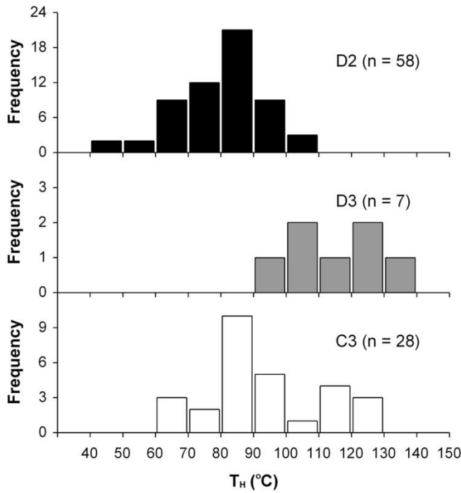
Figure 5: Histogram of homogenization temperatures for fluid inclusions in the D2 and D3 dolomites and C3 calcite of the Watts Bight Formation.
