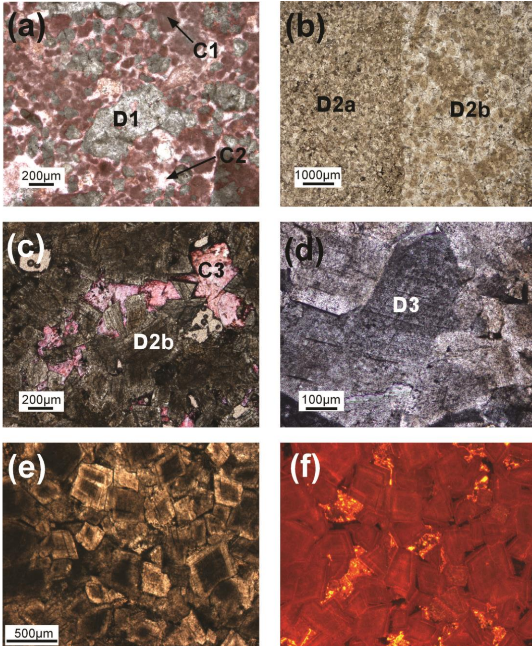
Figure 3: Photomicrographs of the Watts Bight Formation. (a) Stained thin section showing D1 dolomite replacing C1 micrite peloidal and intraclasts; (b) Photomicrograph of D2a and D2 dolomite; (c) Stained thin section showing Fe-poor (pink) and Fe-rich (purple) C3 infilling pores between D2b rhombs; (d) Stained thin section with D3 dolomite showing undulose extinction; (e) D2b dolomite; (f) Same view as (a) under cathodoluminescence showing zoned orange/red luminescence of D2 dolomite and yellow fluorescence of C3 infilling pores.
