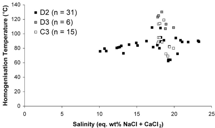
Figure 6: Bivariate plot of homogenization temperature vs. salinity for fluid inclusions in the D2 and D3 dolomites and C3 calcite of the Watts Bight Formation.
