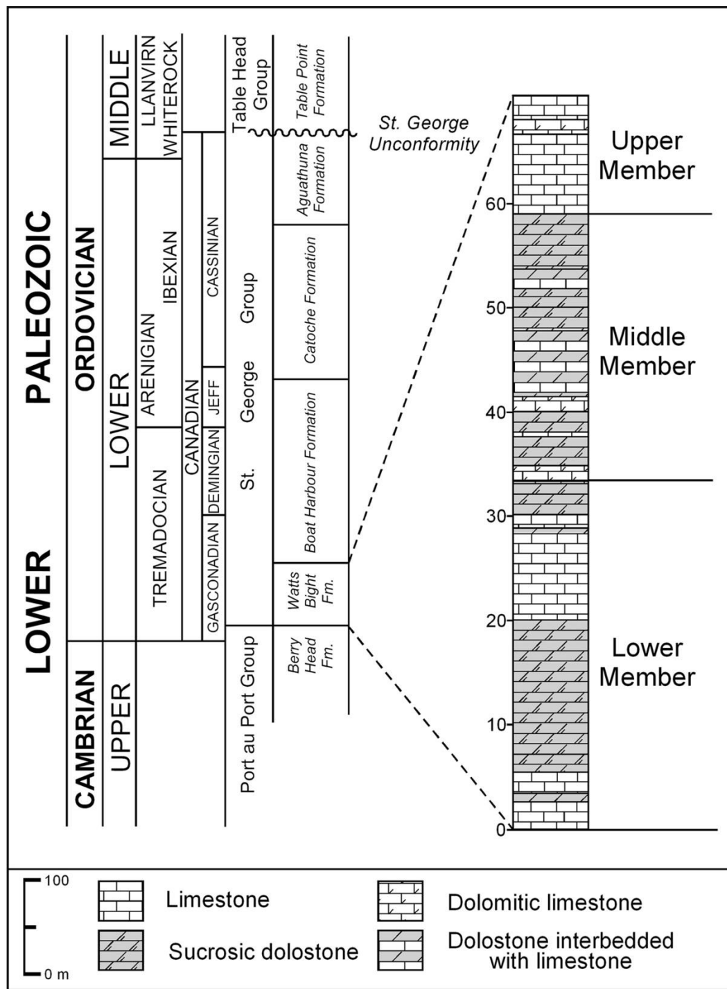
Figure 2: Simplified lithostratigraphy of the St. George Group, Port au Port peninsula with detailed section of the Watts Bight Formation showing the distribution of dolostones and limestones (adapted from Knight et al. 2008).
