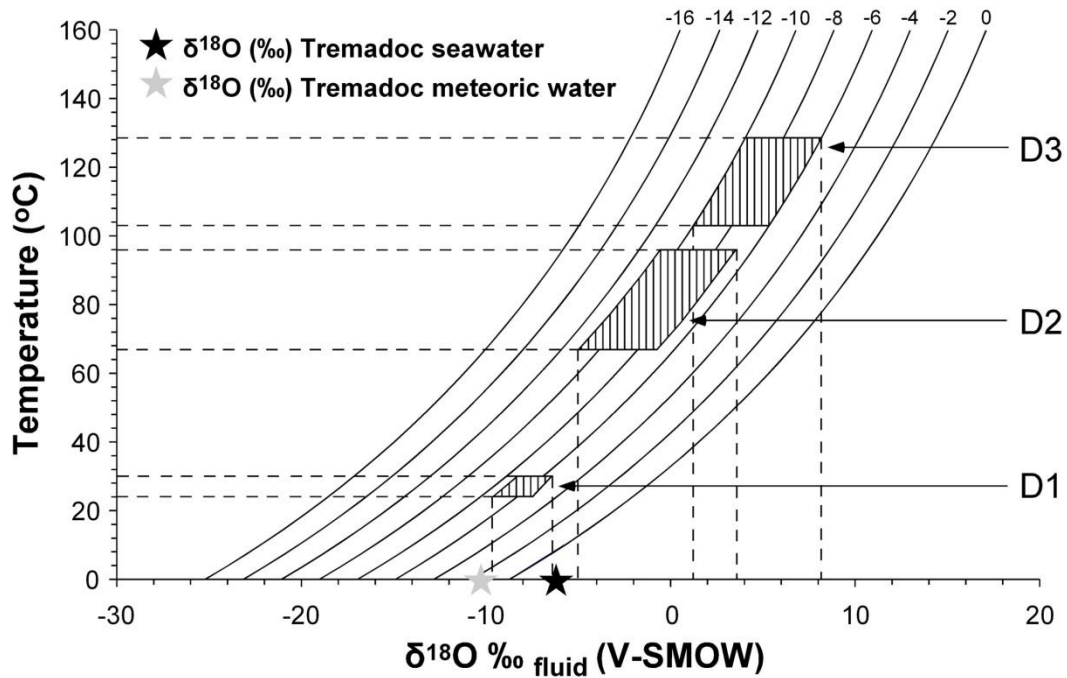
Figure 9: Temperature vs. \delta^{18}\text{O}_{\text{fluid}} for various \delta^{18}\text{O}_{\text{dolomite}} derived from the fractionation equation: 10^3 \ln \alpha_{\text{dolomite-water}} = 3.2 \times 10^6 T^{-2} - 3.3 (Lands, 1983). Hatched areas represent range of temperatures and \delta^{18}\text{O} for various dolomite generations (D1, D2, D3). Values for Tremadoc seawater from Shields et al. (2003). See text for details.
