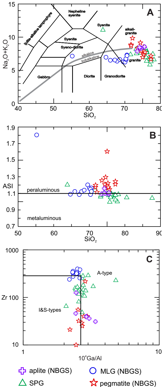
Figure 3. A) Rock types (after Cox et al. , 1979; Wilson, 1989); B) Aluminum saturation index ( ASI = Al/(Ca - 1.67P + Na + K) ) of the granitoids (after Shand, 1922); C) Type of granitoids (Whalen et al. , 1987).
