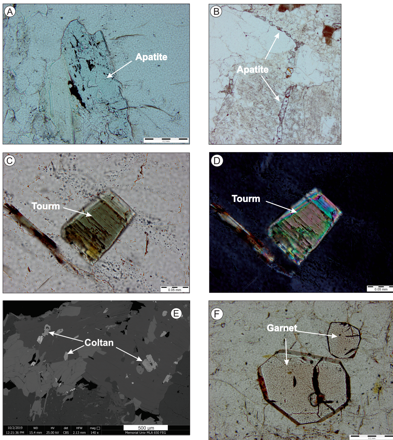
Plate 5. A) Subhedral apatite in pegmatite; B) Anhedral apatite along grain boundaries of quartz and feldspars in pegmatite; C) Tourmaline in pegmatite; D) Same as C under crossed polars; E) Back-scattered electron image of coltan in pegmatite; F) Zoned garnet in aplite. Key: Tourm—tourmaline. Author correction to Plate 5E: Replaced BSE image and caption, May, 2024.
