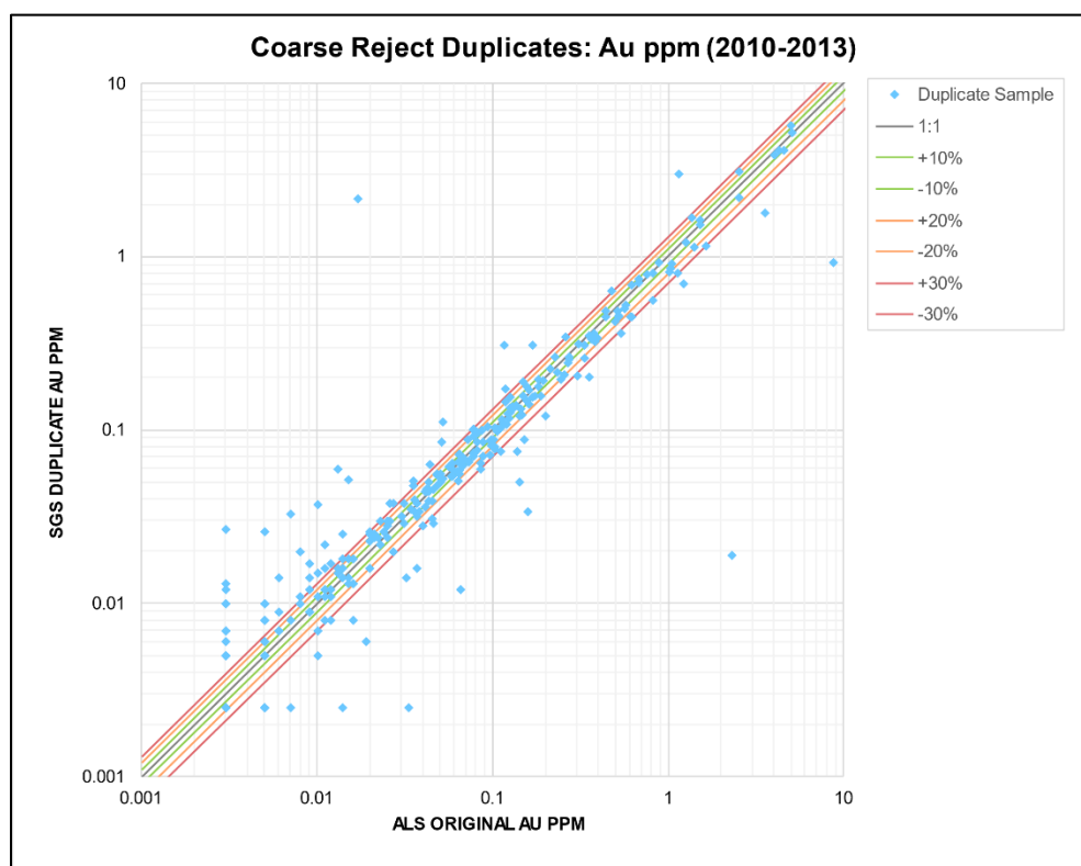
Figure 11-1 Log X-Y Plot of Coarse Reject Duplicate Samples for Gold (2010 – 2013)
