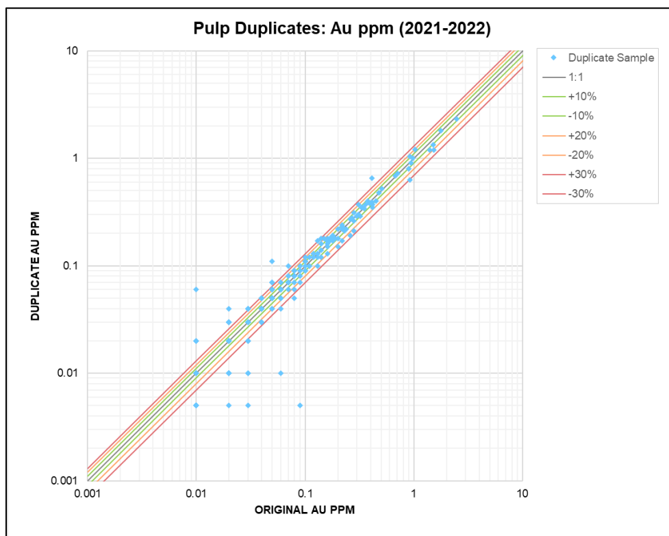
Figure 11-10 Log X-Y Plot of Pulp Duplicate Samples for Gold (2021 – 2022)
