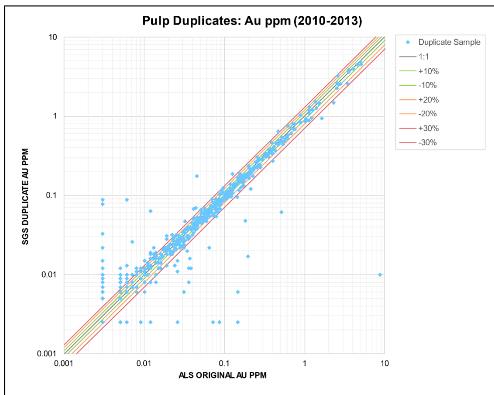
Figure 11-2 Log X-Y Plot of Pulp Duplicate Samples for Gold (2010 – 2013)
