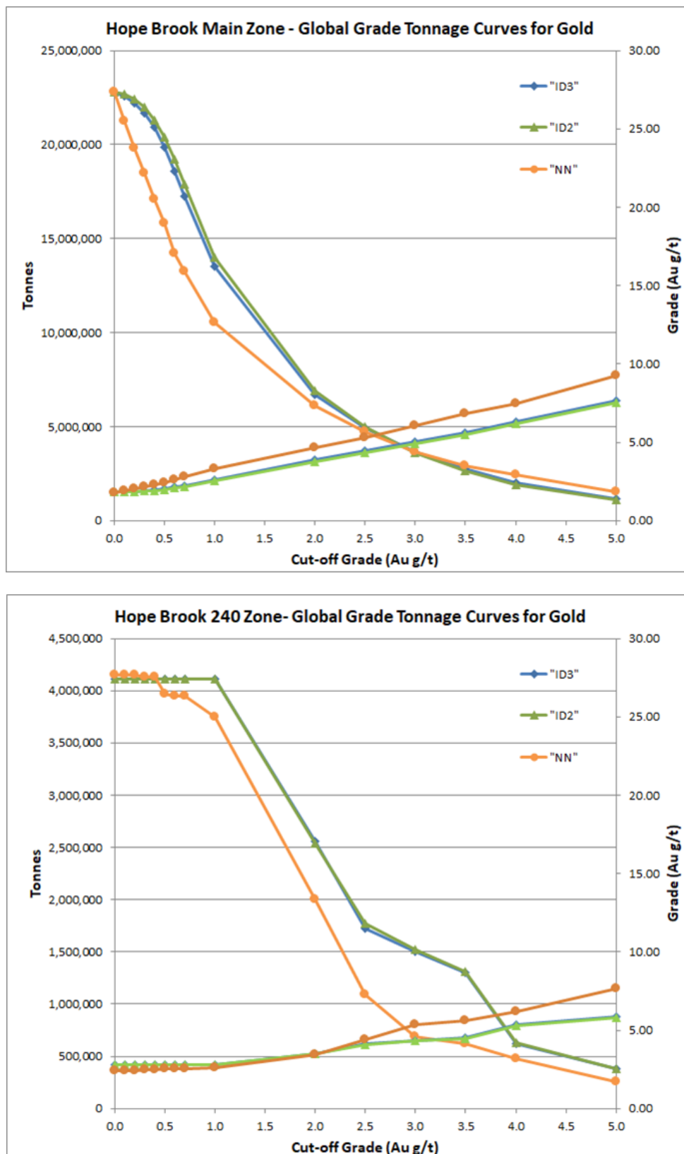
Figure 14-13 Comparison of ID 3 , ID 2 & NN Models for the HB Deposit In-pit and Underground Mineral Resource
