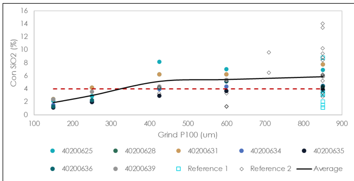
Figure 13—6: 2012 HLS Testwork - Impact of Grind Size on Silica Rejection via Gravity Separation for HMOX Samples
