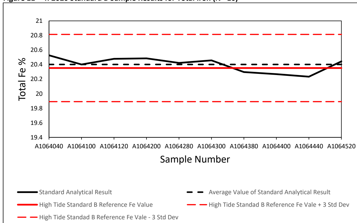
Figure 11—4: 2020 Standard B Sample Results for Total Iron (N= 10)
