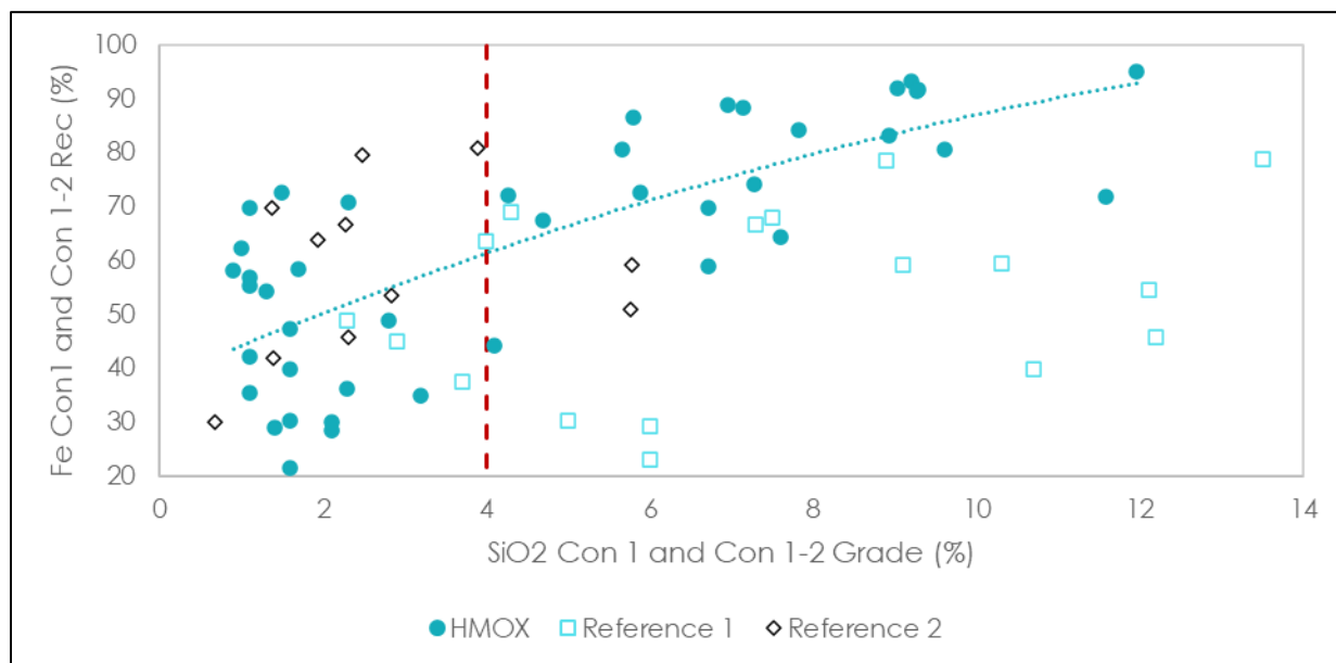
Figure 13—12: 2020 WT Testwork Results - Iron Recovery per Sample Type at 425 \mu\text{m}
