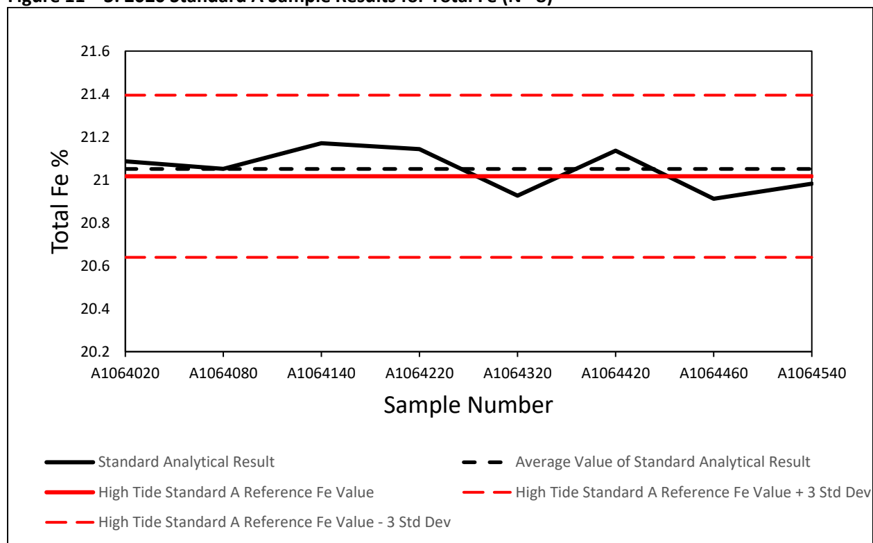
Figure 11—3: 2020 Standard A Sample Results for Total Fe (N= 8)
