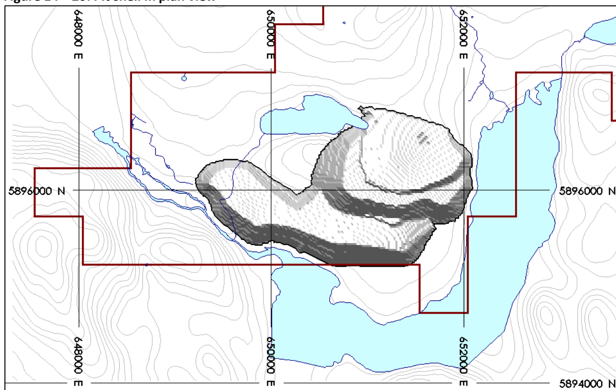
Figure 14—20: Pit shell in plan view
