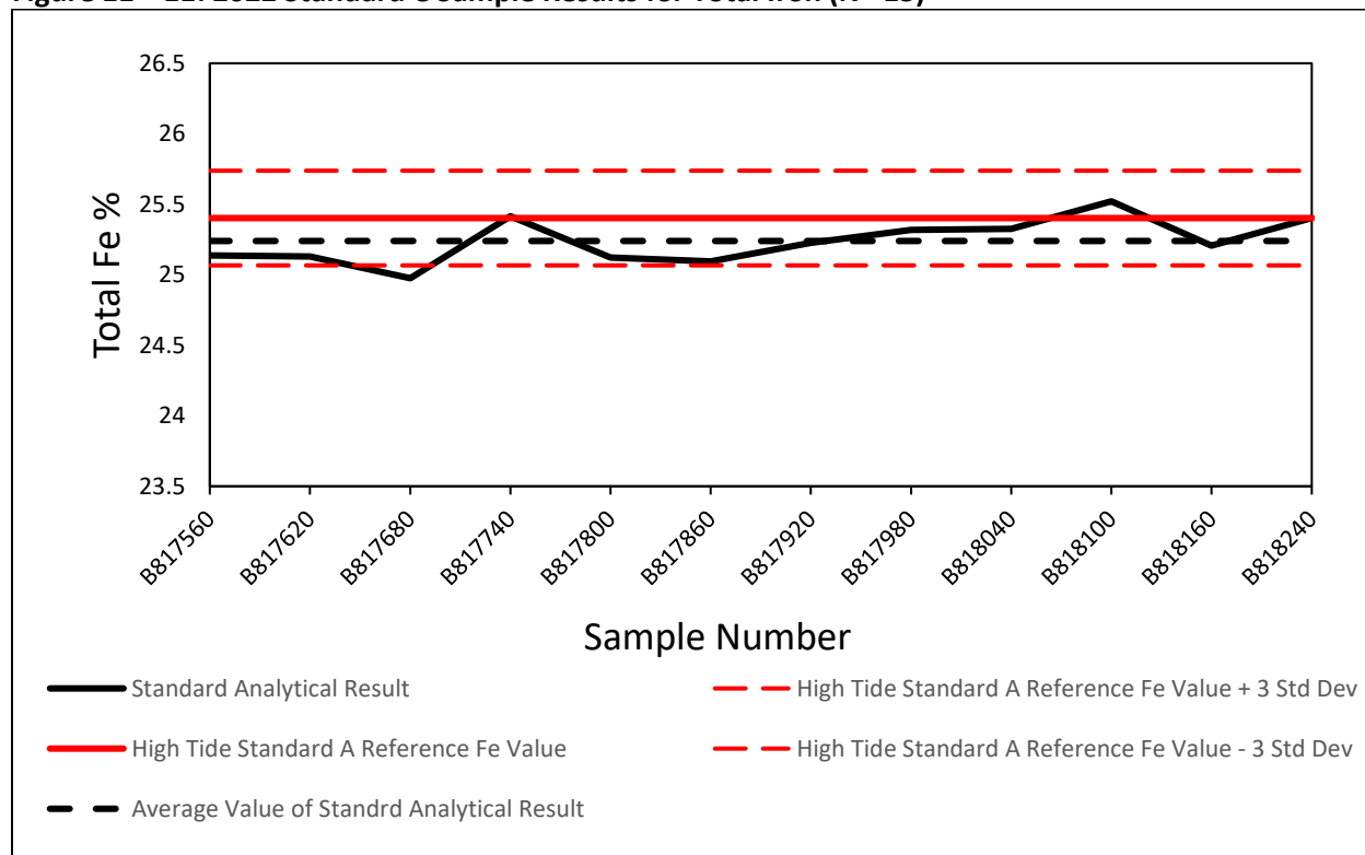
Figure 11—11: 2022 Standard C Sample Results for Total Iron (N= 13)
