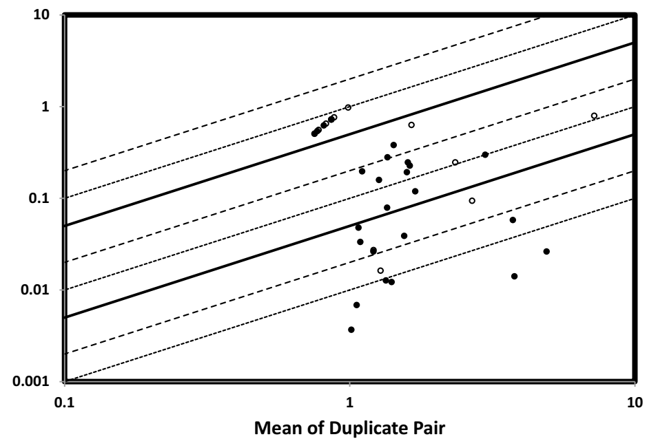
Mo (ICP-OES) / ppm
