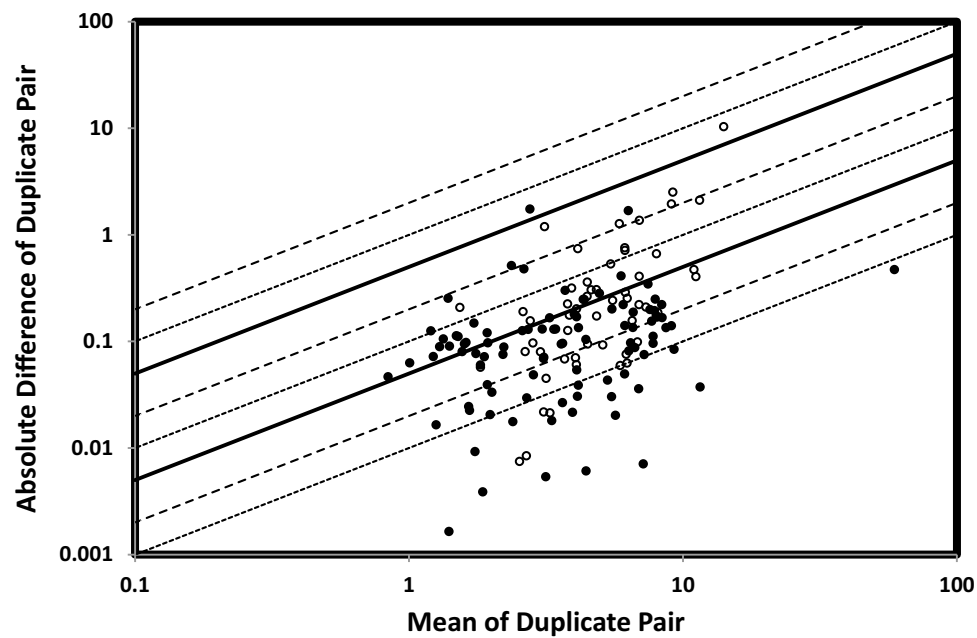
Dy (ICP-OES)/ ppm
