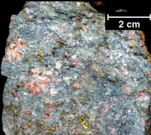
Butler's Pond: intrusion related Cu-Au
