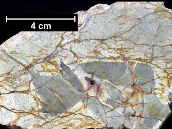
New Fortune (LS) epithermal gold
