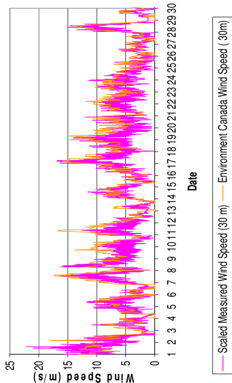
Cartwright Calculated Wind Speed - November
