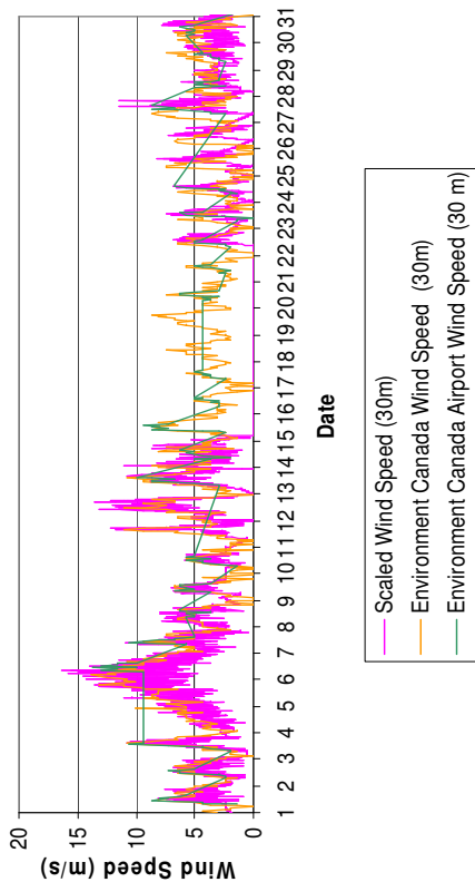
Mary's Harbour Calculated Wind Speed - July
